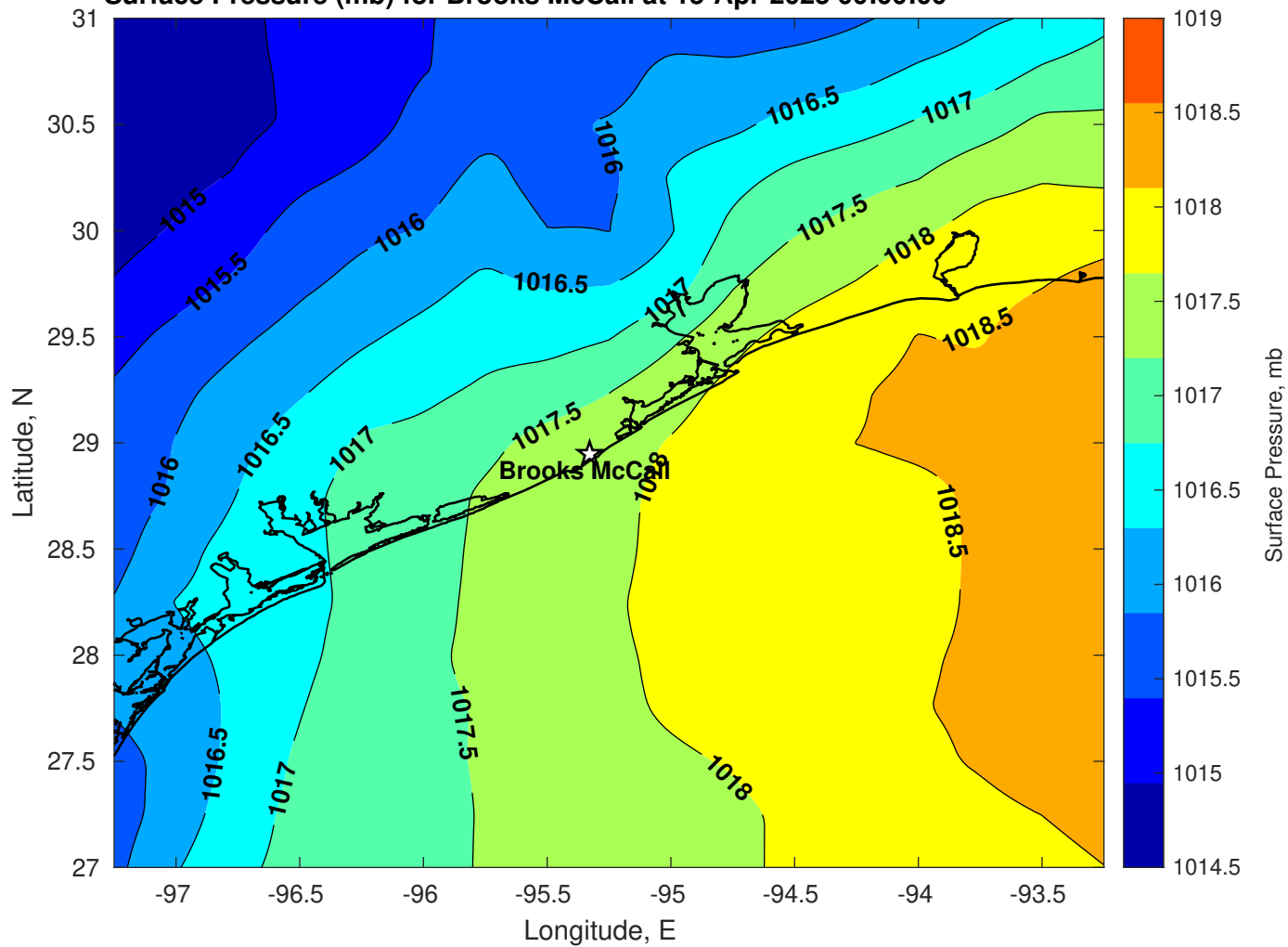
Surface Pressure (mb) for Brooks McCall at 15-Apr-2025 00:00:00
