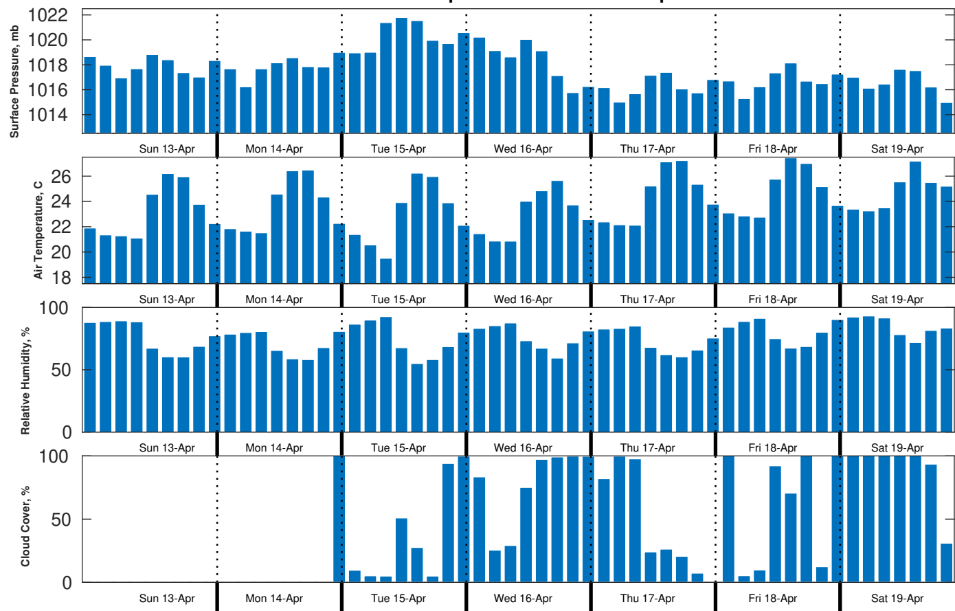
Met Forecast for Brooks McCall from 13-Apr-2025 00:00:00 to 20-Apr-2025 00:00:00
