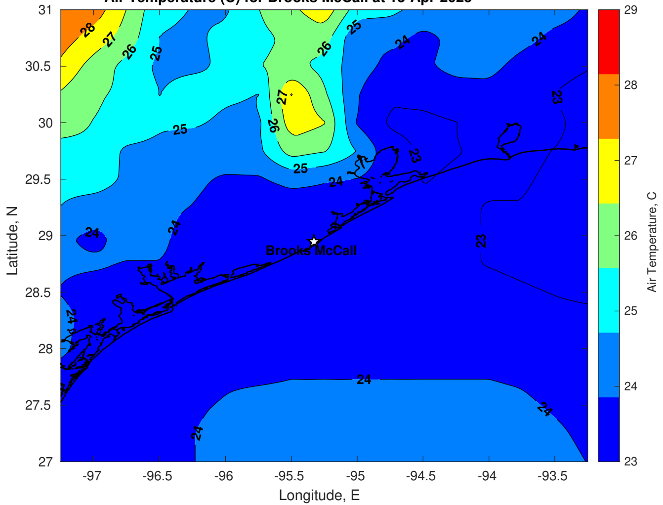
Air Temperature (C) for Brooks McCall at 13-Apr-2025
