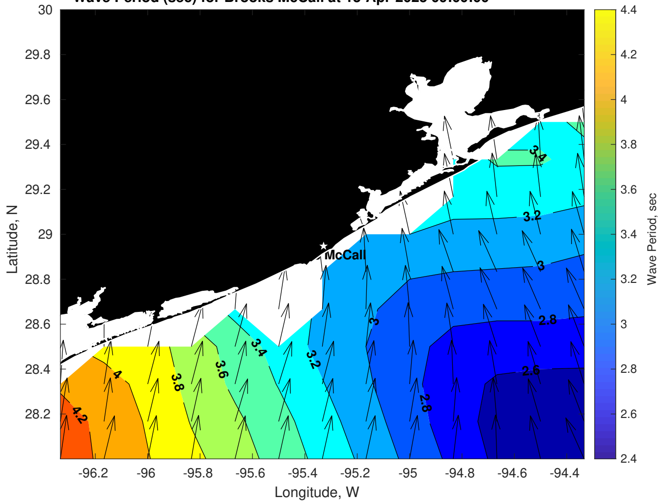
Wave Period (sec) for Brooks McCall at 13-Apr-2025 09:00:00
