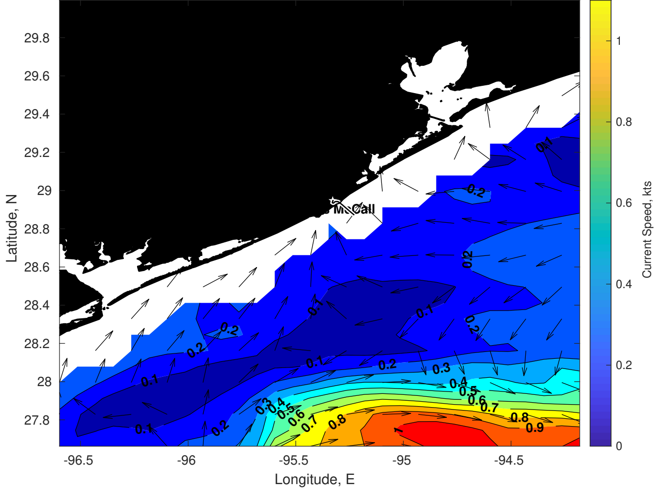
Surface Currents for Brooks McCall at 12-Apr-2025 00:00:00
