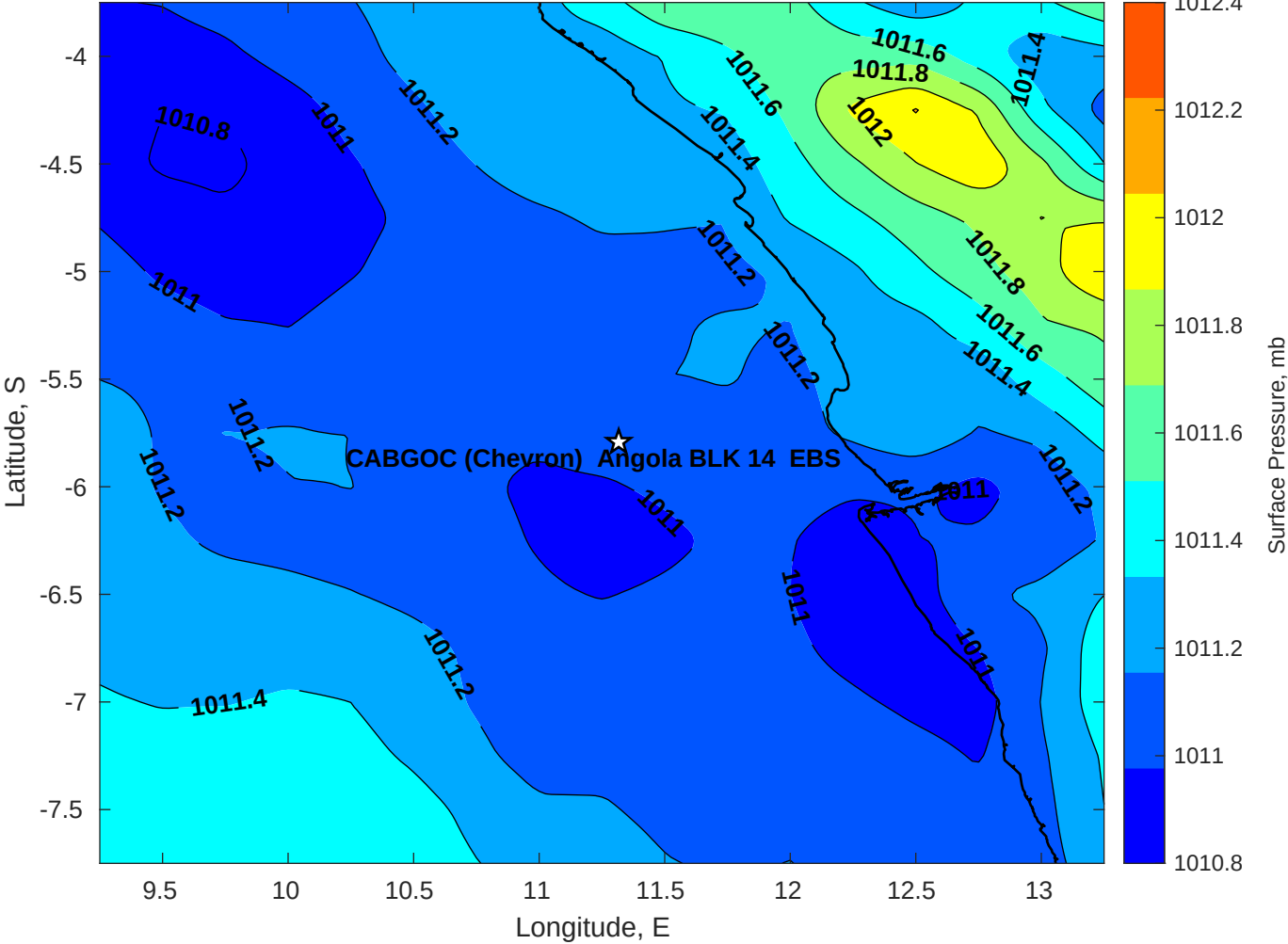
Surface Pressure (mb) for CABGOC (Chevron) Angola BLK 14 EBS at 14-Apr-2025 00:00:00
