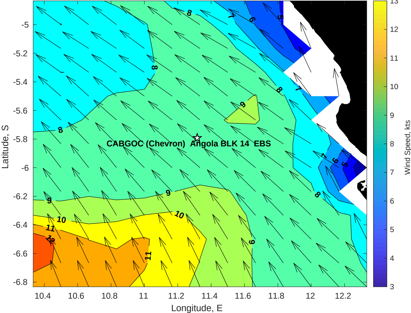
Winds (kts) for CABGOC (Chevron) Angola BLK 14 EBS at 13-Apr-2025 09:00:00
