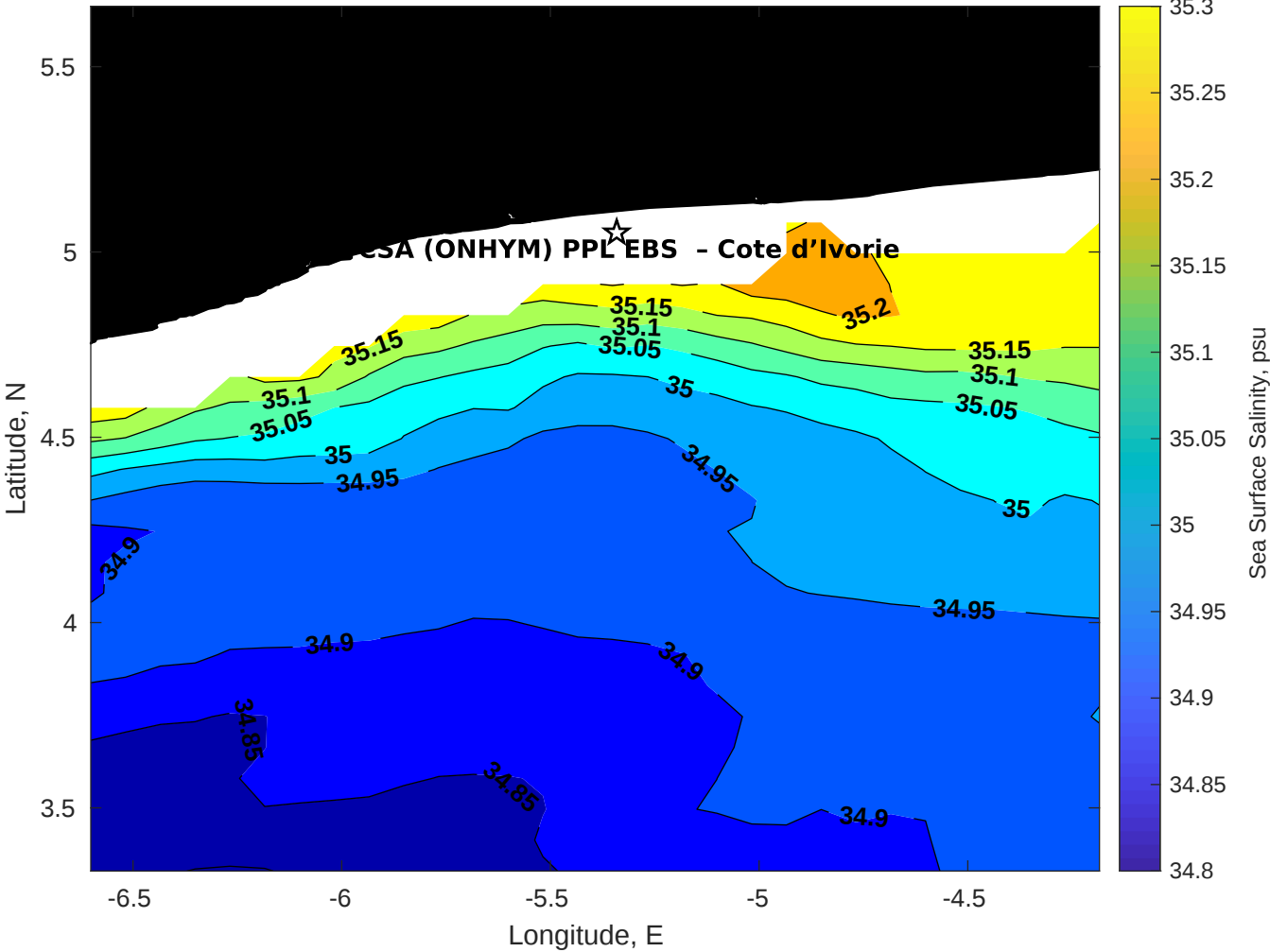
Surface Salinity for CSA (ONHYM) PPL EBS - Cote d'Ivoire at 12-Apr-2025 00:00:00
