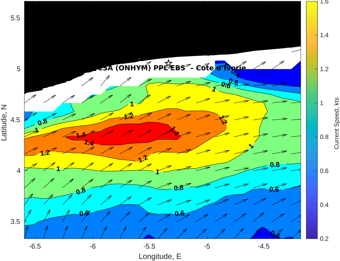
Surface Currents for CSA (ONHYM) PPL EBS - Cote d'Ivoire at 12-Apr-2025 00:00:00
