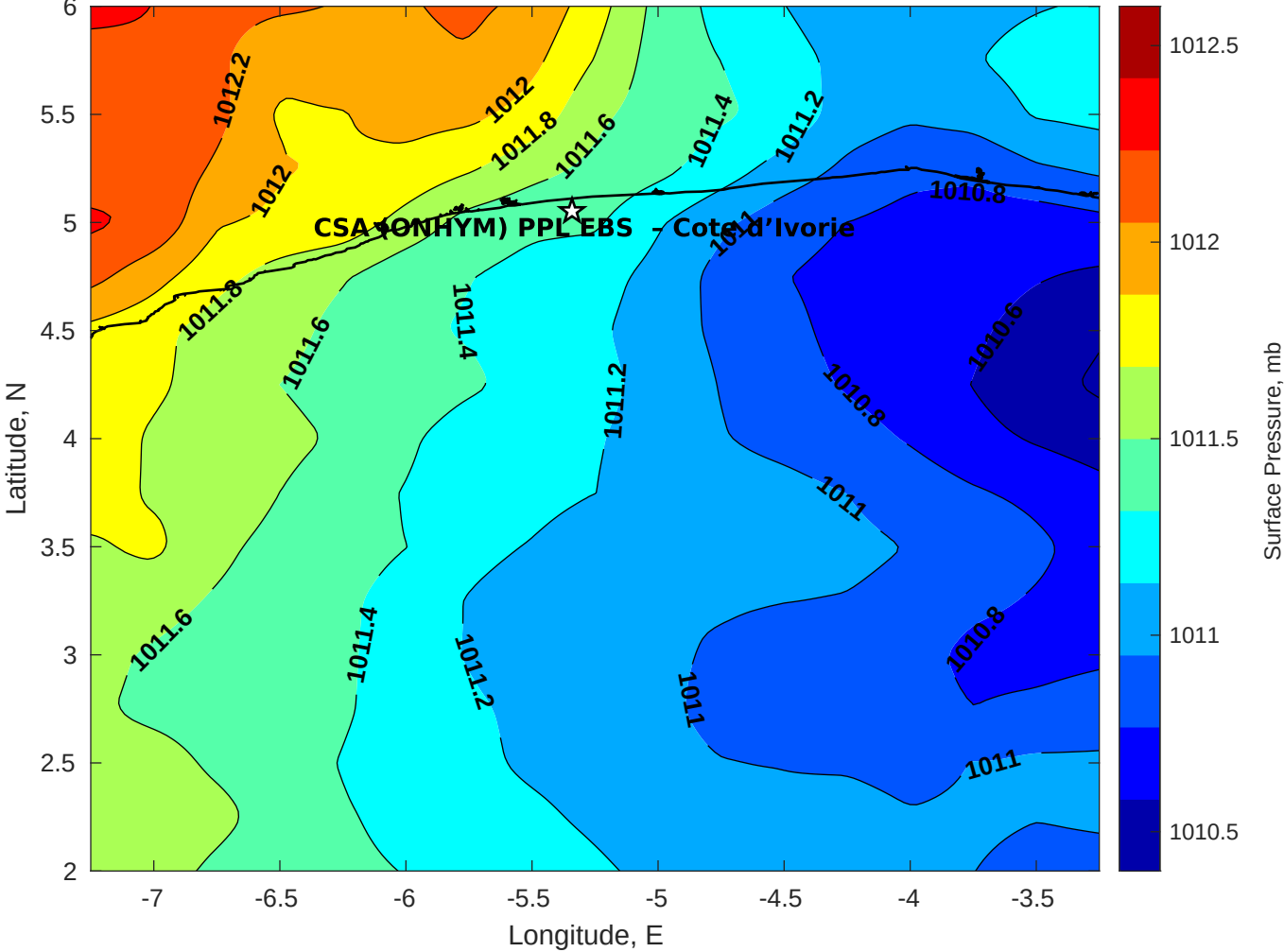
Surface Pressure (mb) for CSA (ONHYM) PPL EBS - Cote d'Ivoire at 15-Apr-2025 00:00:00
