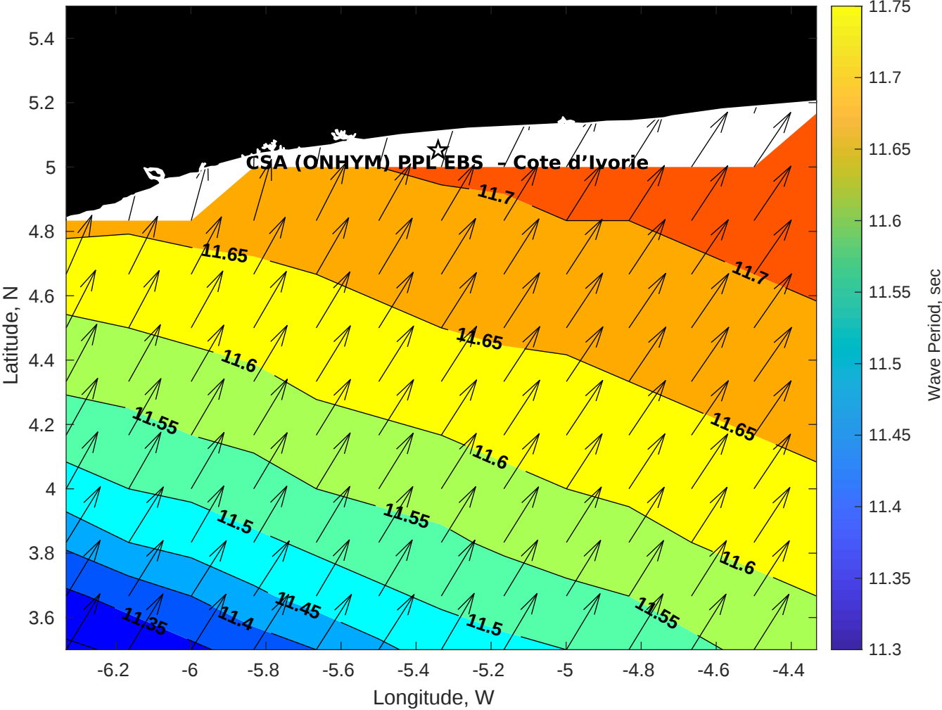
Wave Period (sec) for CSA (ONHYM) PPL EBS - Cote d'Ivoire at 13-Apr-2025 09:00:00
