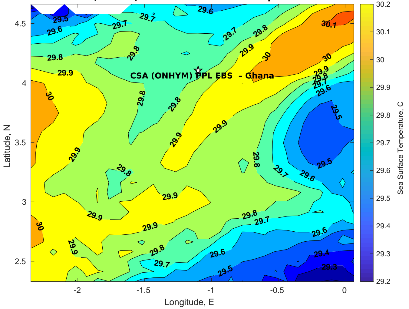
SST for CSA (ONHYM) PPL EBS - Ghana at 12-Apr-2025 00:00:00
