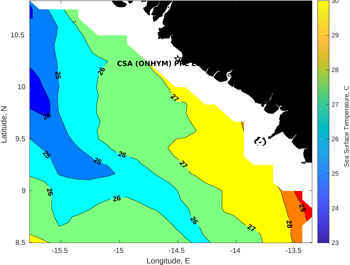
SST for CSA (ONHYM) PPL EBS - Guinea at 12-Apr-2025 00:00:00
