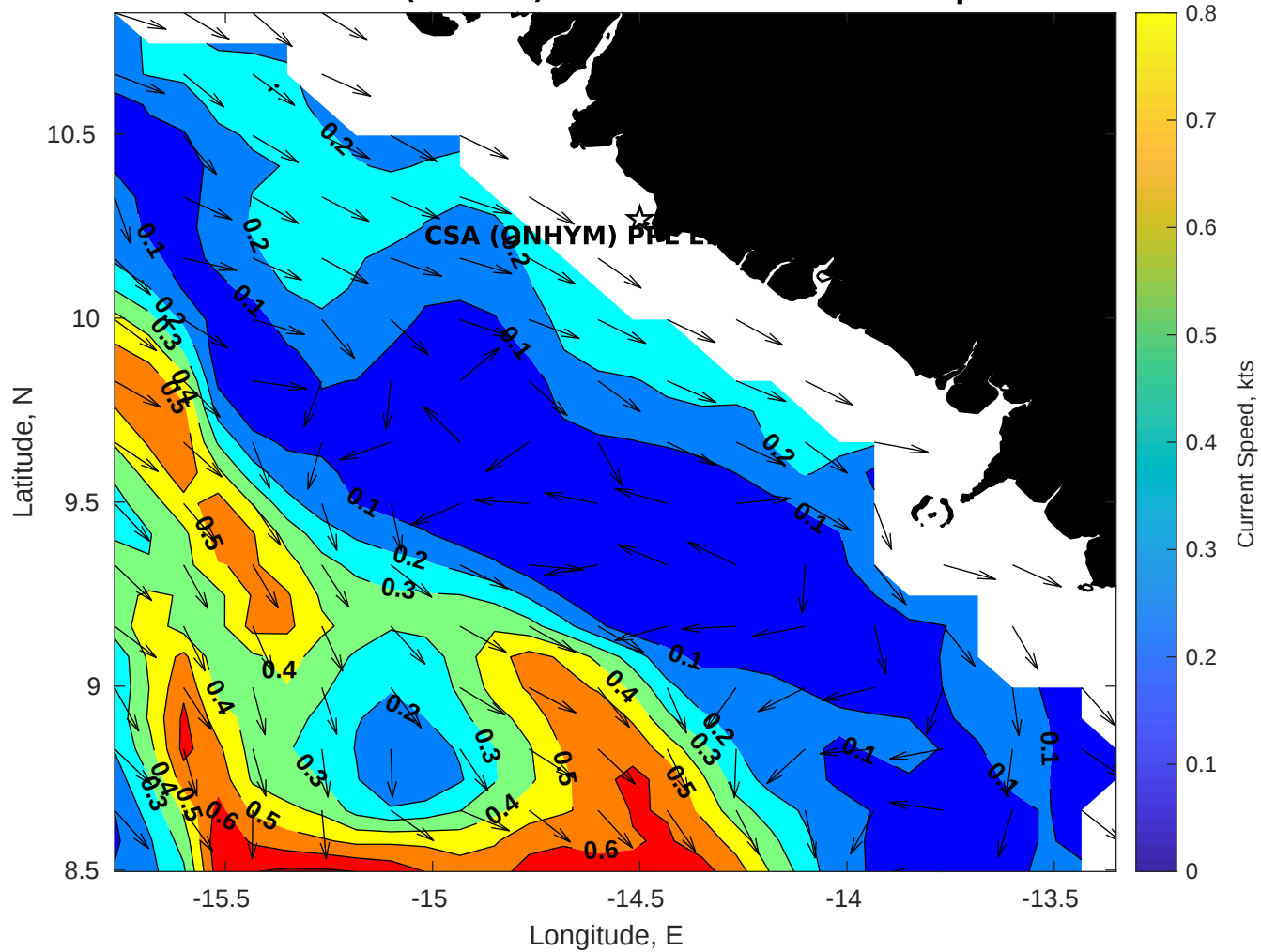
Surface Currents for CSA (ONHYM) PPL EBS - Guinea at 12-Apr-2025 00:00:00
