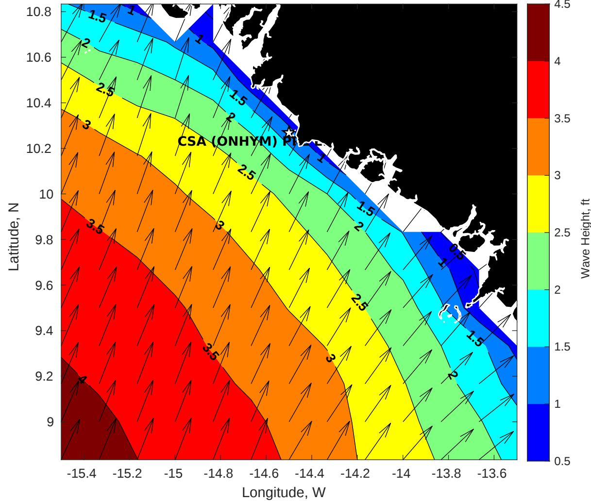
Wave Height (ft) for CSA (ONHYM) PPL EBS - Guinea at 13-Apr-2025 09:00:00
