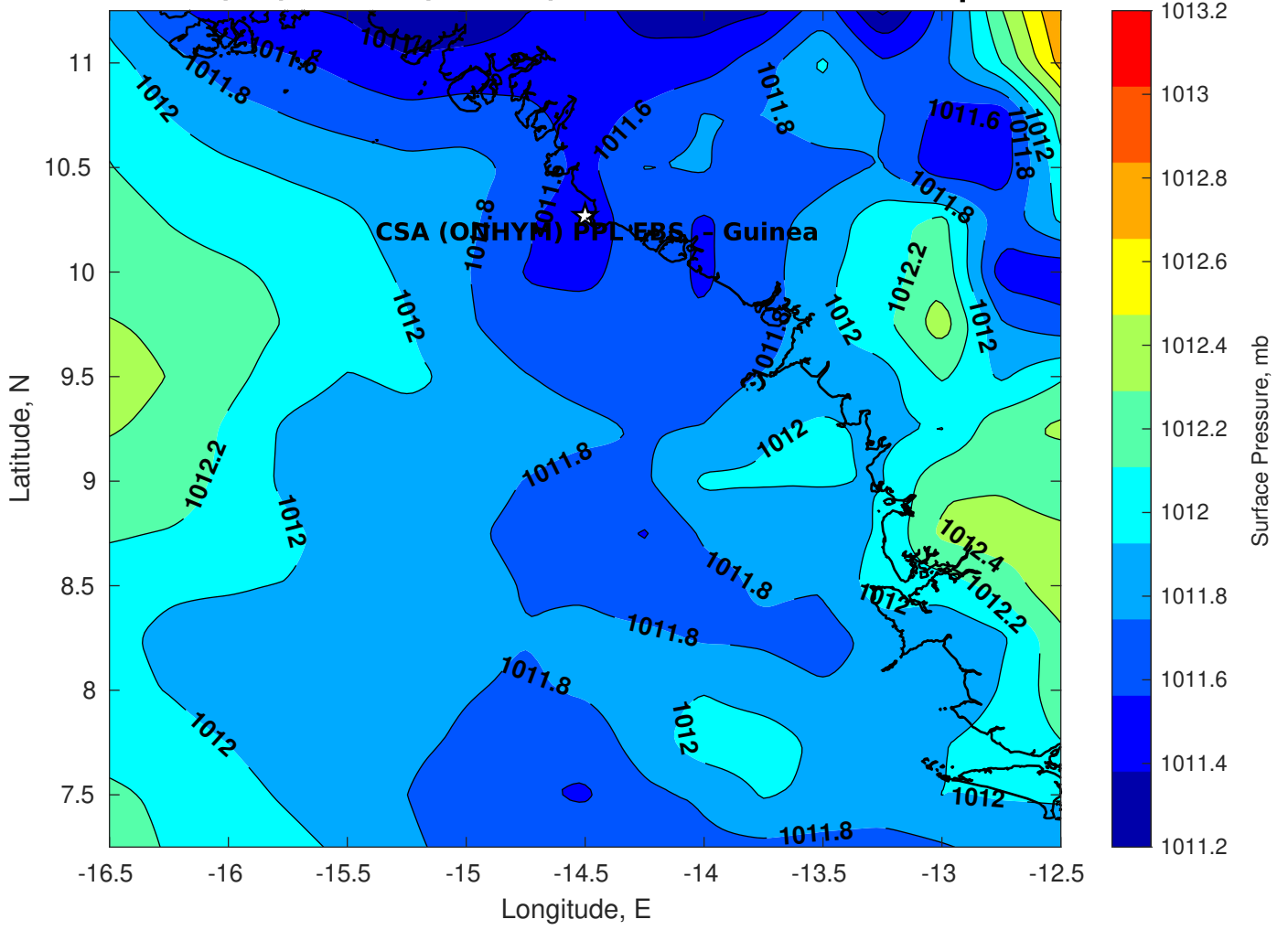
Surface Pressure (mb) for CSA (ONHYM) PPL EBS - Guinea at 13-Apr-2025 00:00:00
