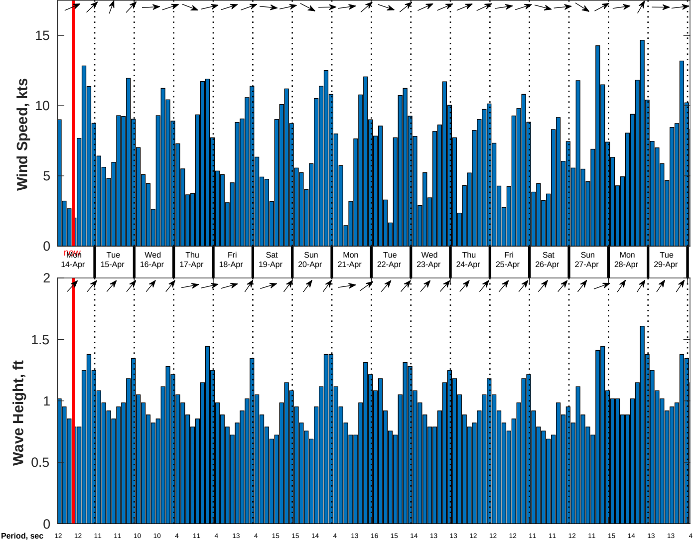
Wind & Wave Forecast for CSA (ONHYM) PPL EBS - Guinea from 13-Apr-2025 01:00:00 to 29-Apr-2025 01:00:00
