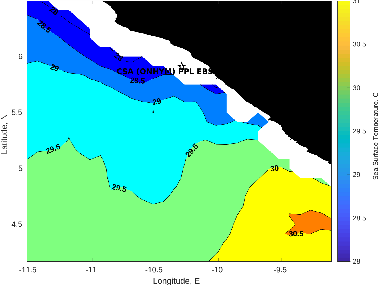
SST for CSA (ONHYM) PPL EBS - Liberia at 12-Apr-2025 00:00:00
