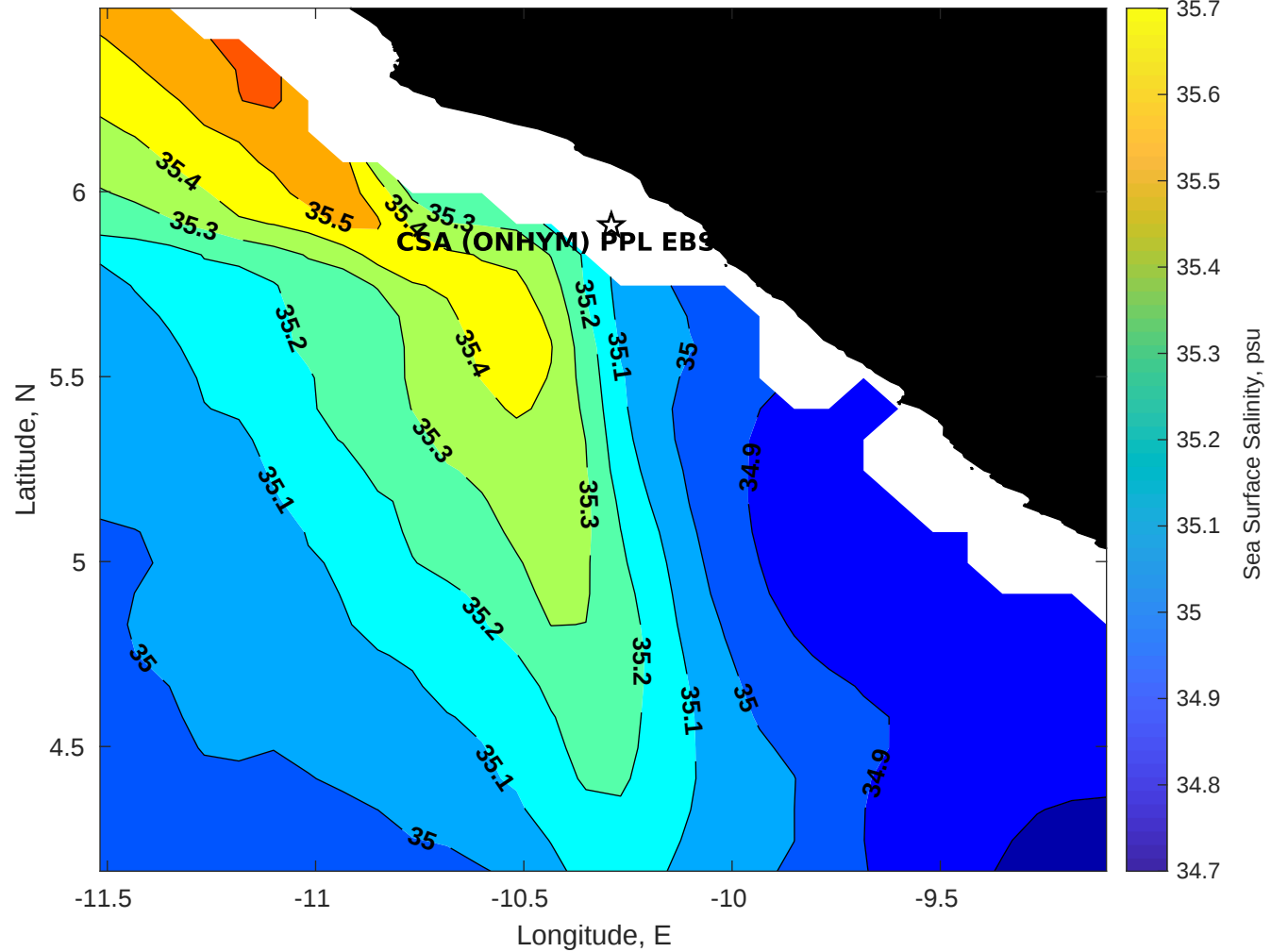
Surface Salinity for CSA (ONHYM) PPL EBS - Liberia at 12-Apr-2025 00:00:00
