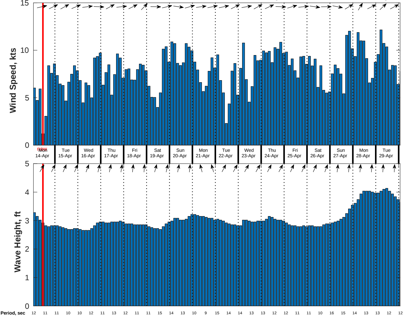
Wind & Wave Forecast for CSA (ONHYM) PPL EBS - Liberia from 13-Apr-2025 01:00:00 to 29-Apr-2025 01:00:00
