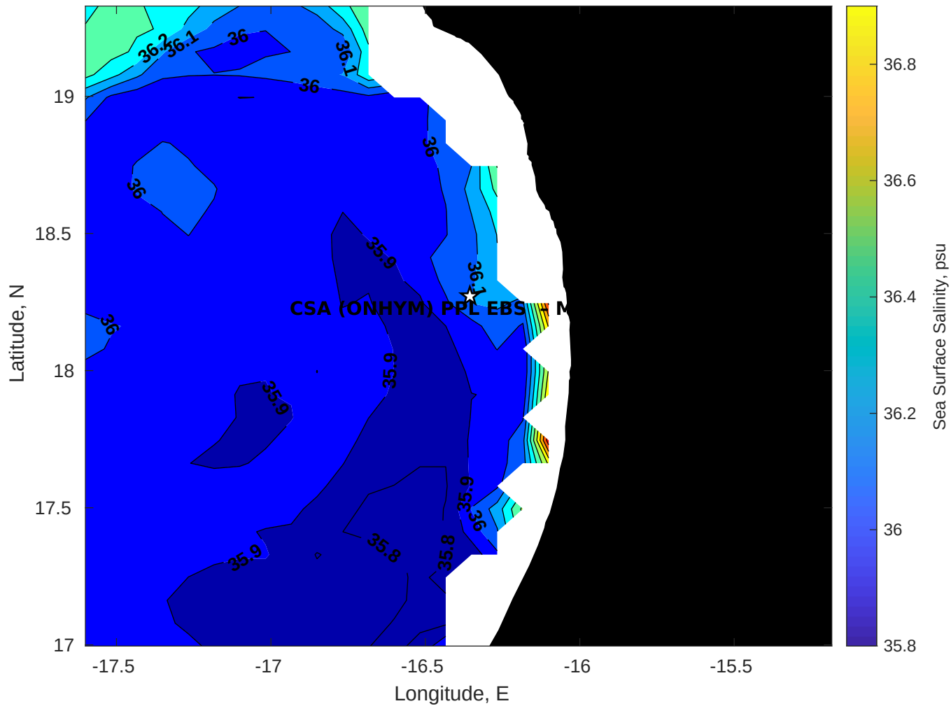
Surface Salinity for CSA (ONHYM) PPL EBS - Mauritania at 12-Apr-2025 00:00:00
