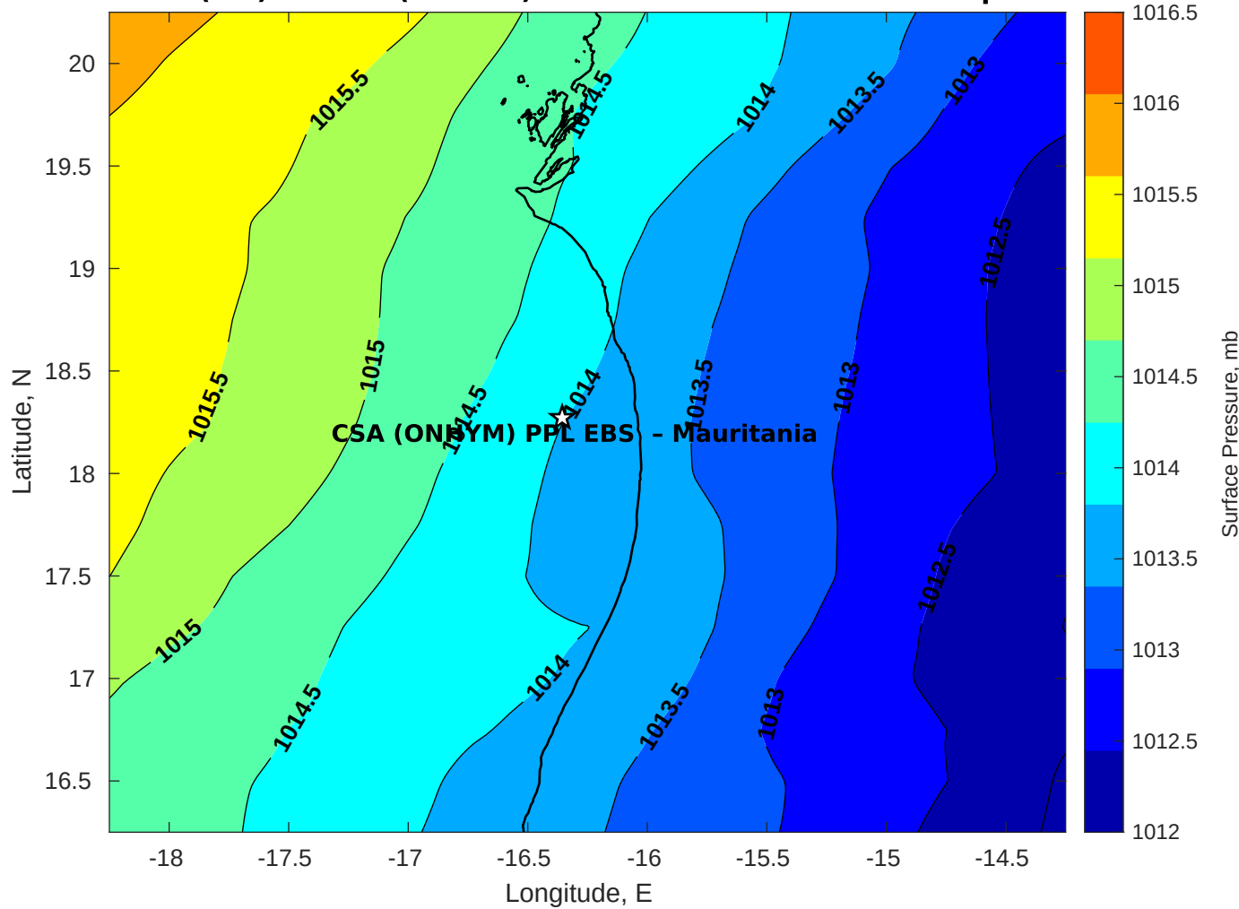
Surface Pressure (mb) for CSA (ONHYM) PPL EBS - Mauritania at 13-Apr-2025 00:00:00
