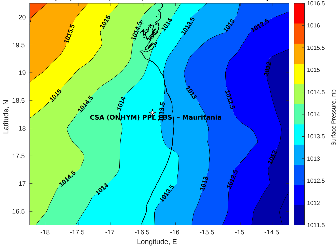
Surface Pressure (mb) for CSA (ONHYM) PPL EBS - Mauritania at 14-Apr-2025 00:00:00
