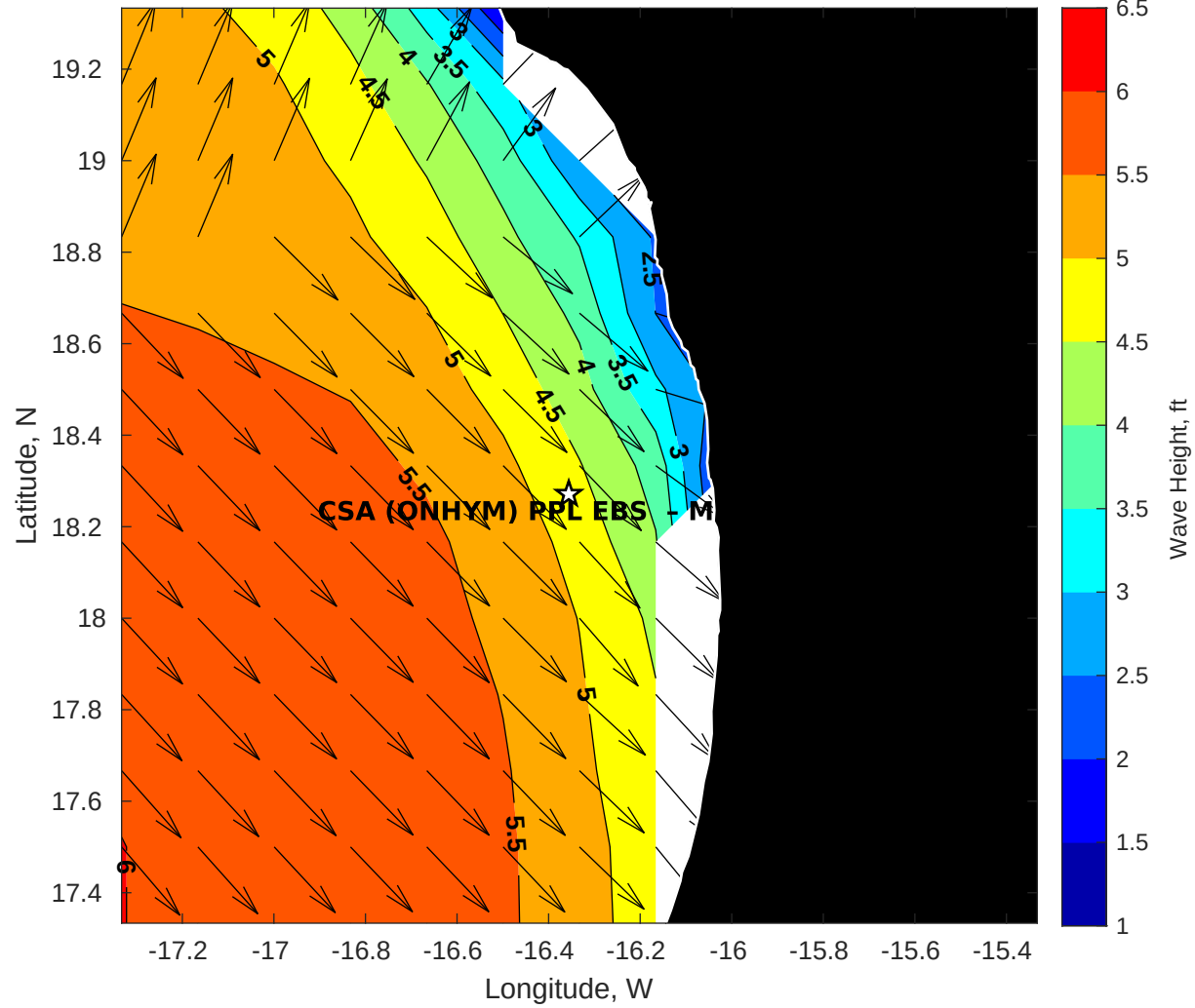
Wave Height (ft) for CSA (ONHYM) PPL EBS - Mauritania at 13-Apr-2025 09:00:00
