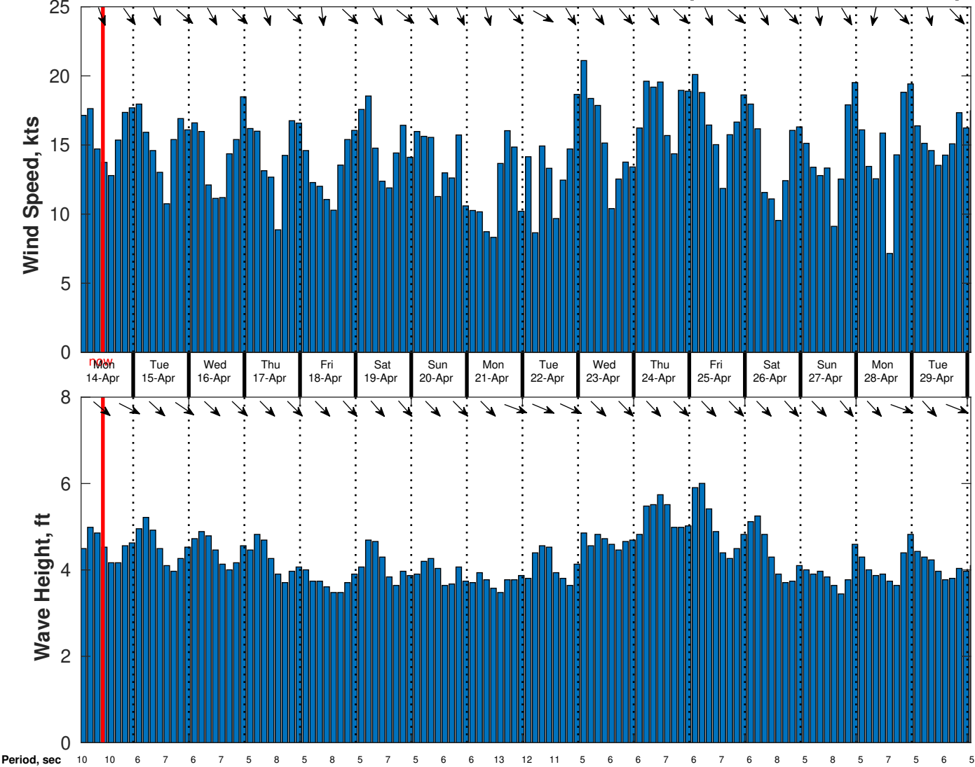
Wind & Wave Forecast for CSA (ONHYM) PPL EBS - Mauritania from 13-Apr-2025 01:00:00 to 29-Apr-2025 01:00:00
