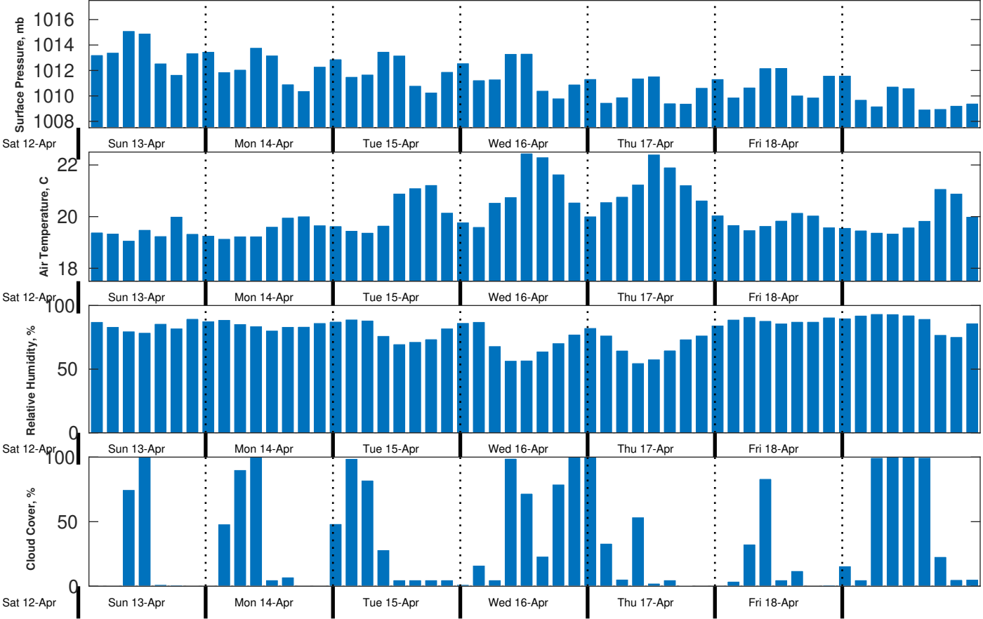
Met Forecast for CSA (ONHYM) PPL EBS - Mauritania from 13-Apr-2025 00:00:00 to 20-Apr-2025 00:00:00
