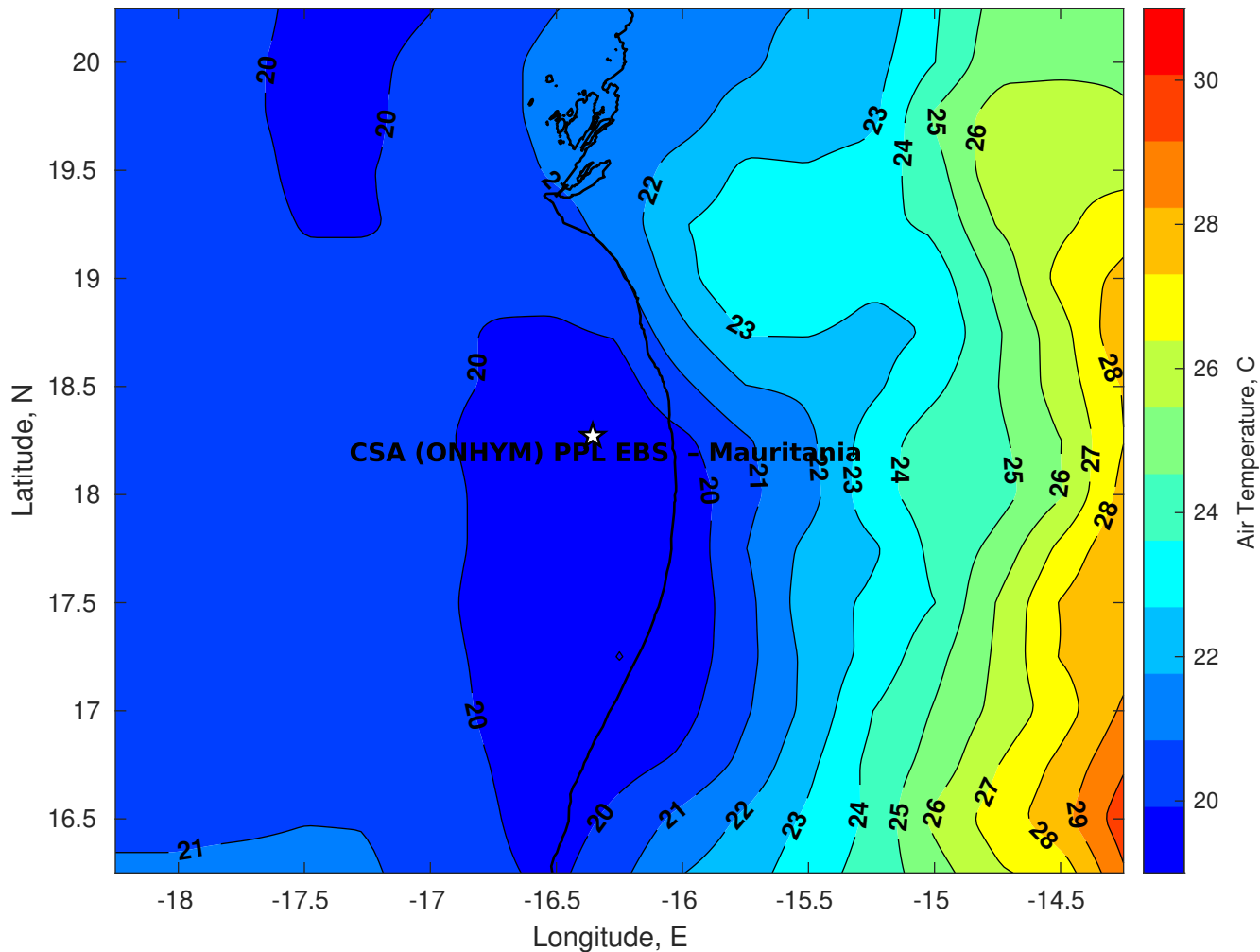
Air Temperature (C) for CSA (ONHYM) PPL EBS - Mauritania at 13-Apr-2025
