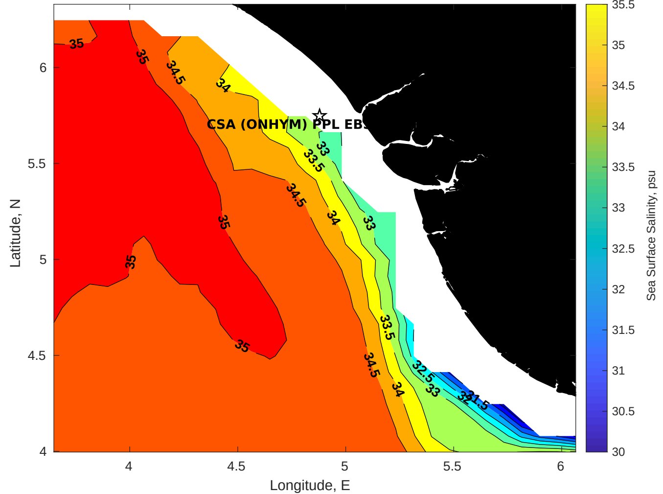
Surface Salinity for CSA (ONHYM) PPL EBS - Nigeria at 12-Apr-2025 00:00:00
