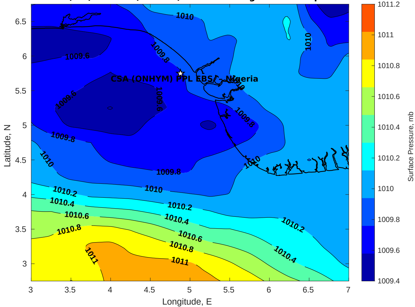
Surface Pressure (mb) for CSA (ONHYM) PPL EBS - Nigeria at 14-Apr-2025 00:00:00
