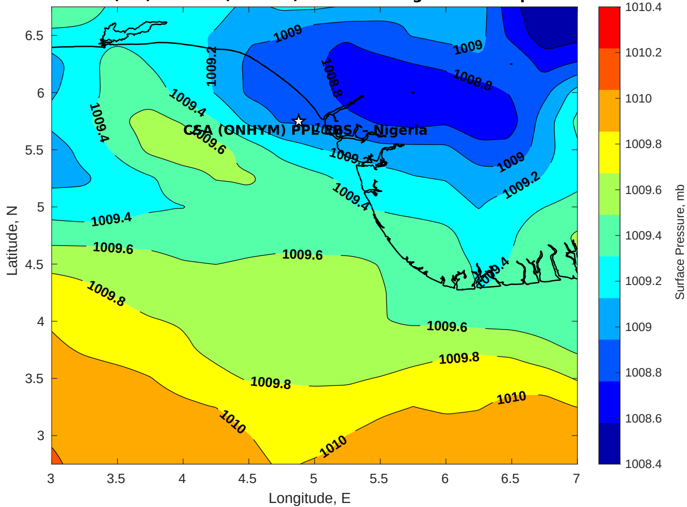
Surface Pressure (mb) for CSA (ONHYM) PPL EBS - Nigeria at 15-Apr-2025 00:00:00
