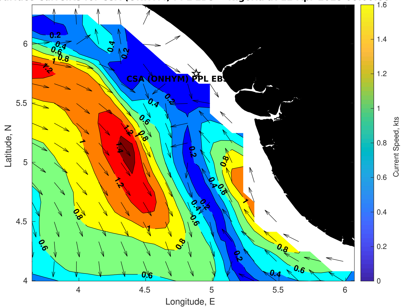
Surface Currents for CSA (ONHYM) PPL EBS - Nigeria at 12-Apr-2025 00:00:00
