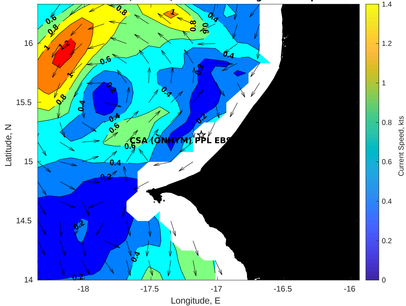
Surface Currents for CSA (ONHYM) PPL EBS - Senegal at 12-Apr-2025 00:00:00
