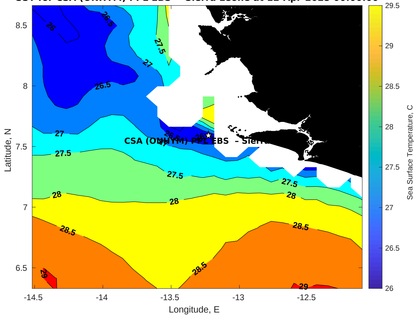
SST for CSA (ONHYM) PPL EBS - Sierra Leone at 12-Apr-2025 00:00:00
