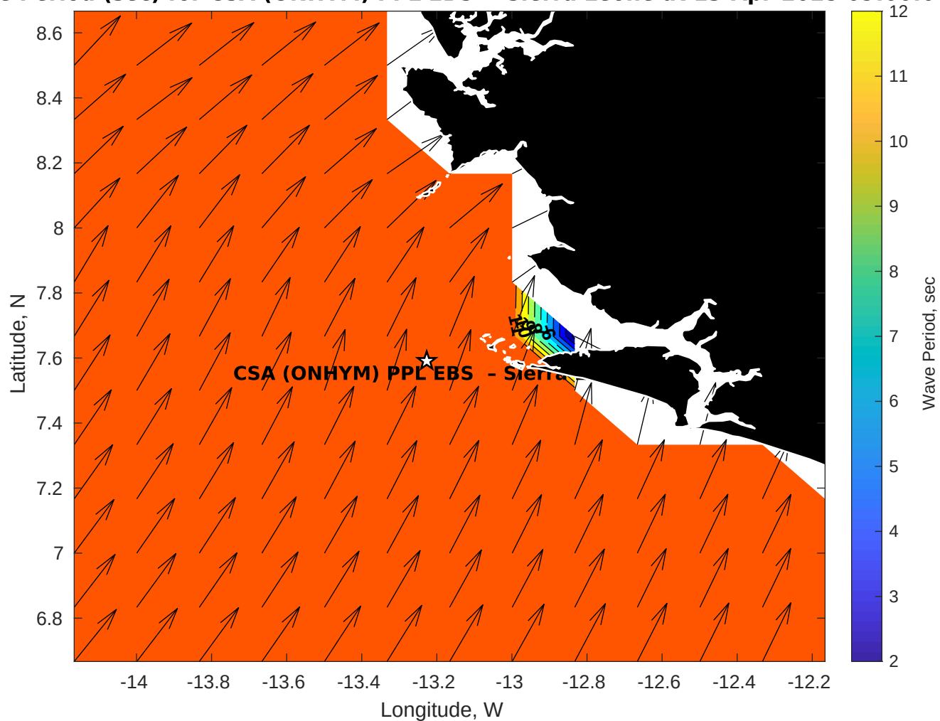
Wave Period (sec) for CSA (ONHYM) PPL EBS - Sierra Leone at 13-Apr-2025 09:00:00
