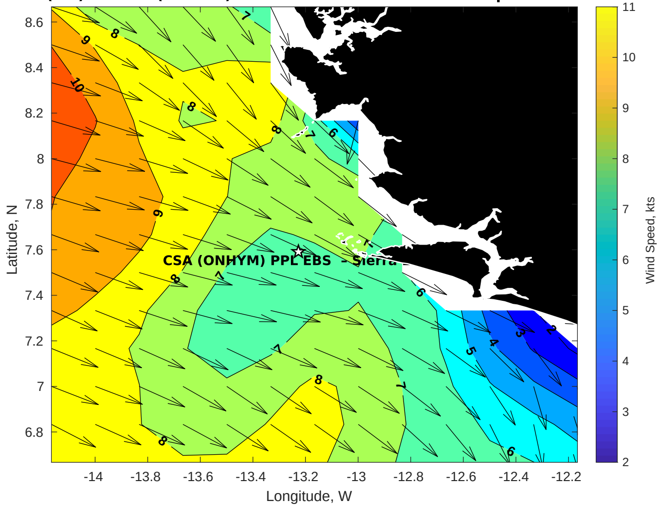
Winds (kts) for CSA (ONHYM) PPL EBS - Sierra Leone at 13-Apr-2025 09:00:00
