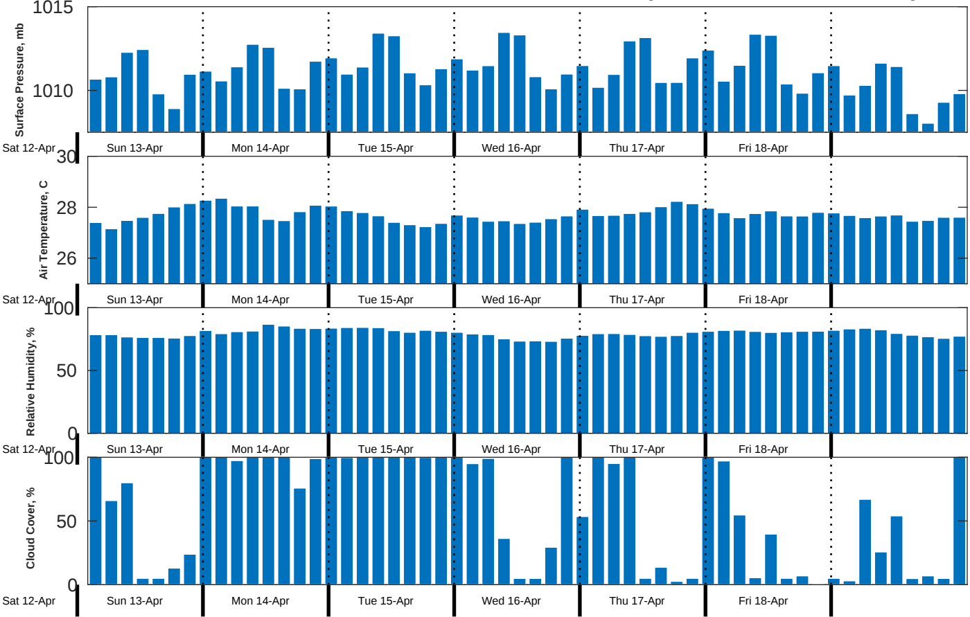
Met Forecast for CSA (ONHYM) PPL EBS - Sierra Leone from 13-Apr-2025 00:00:00 to 20-Apr-2025 00:00:00
