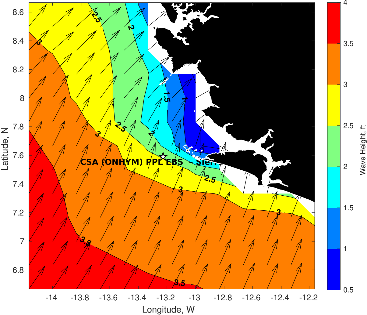
Wave Height (ft) for CSA (ONHYM) PPL EBS - Sierra Leone at 13-Apr-2025 09:00:00
