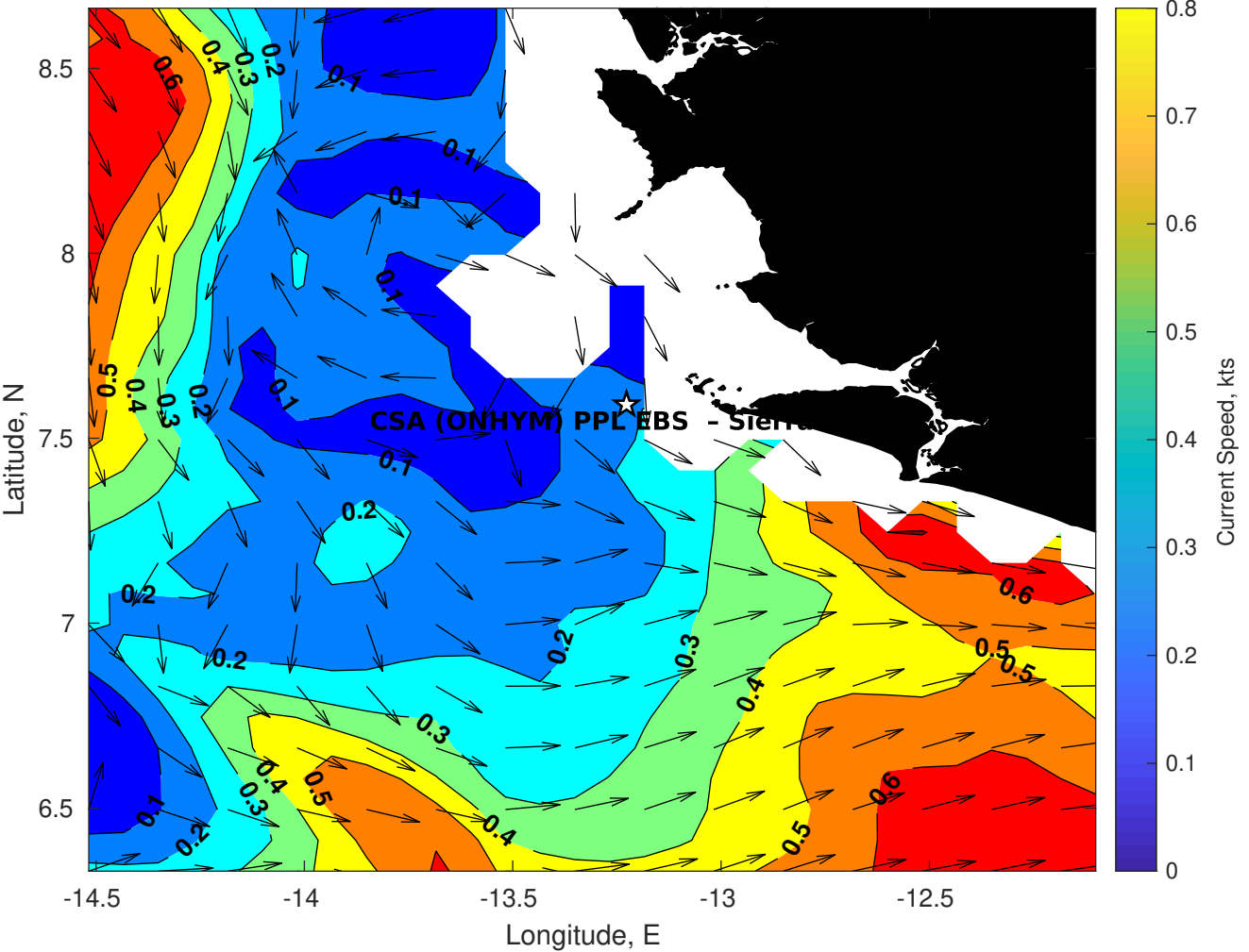
Surface Currents for CSA (ONHYM) PPL EBS - Sierra Leone at 12-Apr-2025 00:00:00
