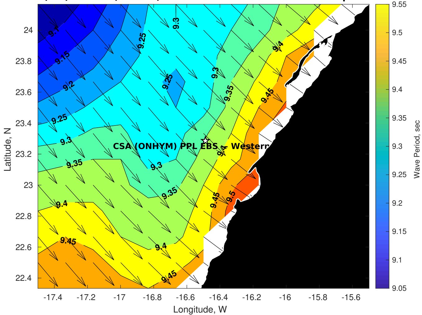
Wave Period (sec) for CSA (ONHYM) PPL EBS - Western Sahara at 13-Apr-2025 09:00:00
