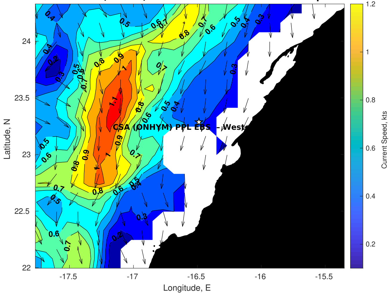
Surface Currents for CSA (ONHYM) PPL EBS - Western Sahara at 12-Apr-2025 00:00:00
