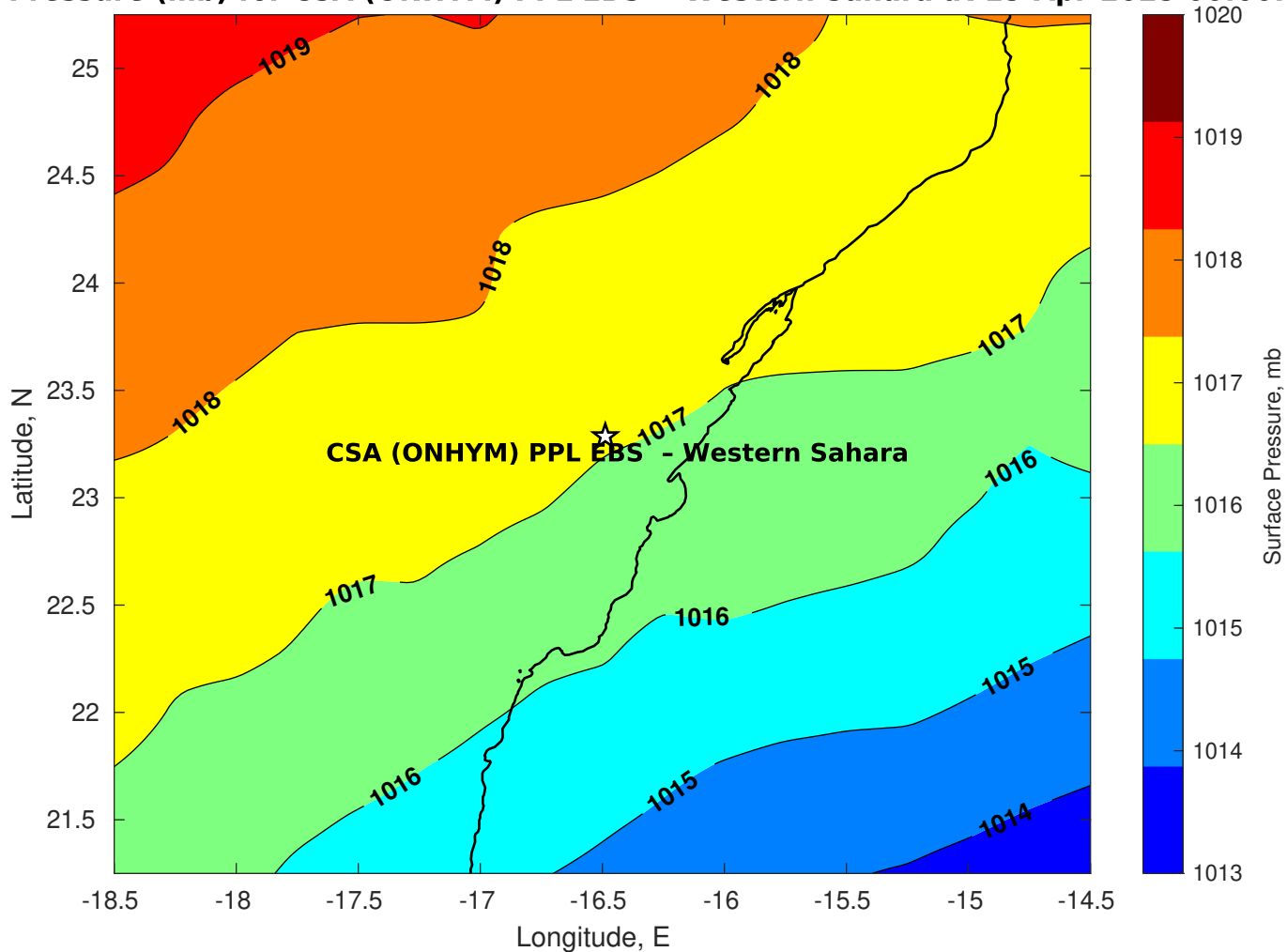
Surface Pressure (mb) for CSA (ONHYM) PPL EBS - Western Sahara at 15-Apr-2025 00:00:00
