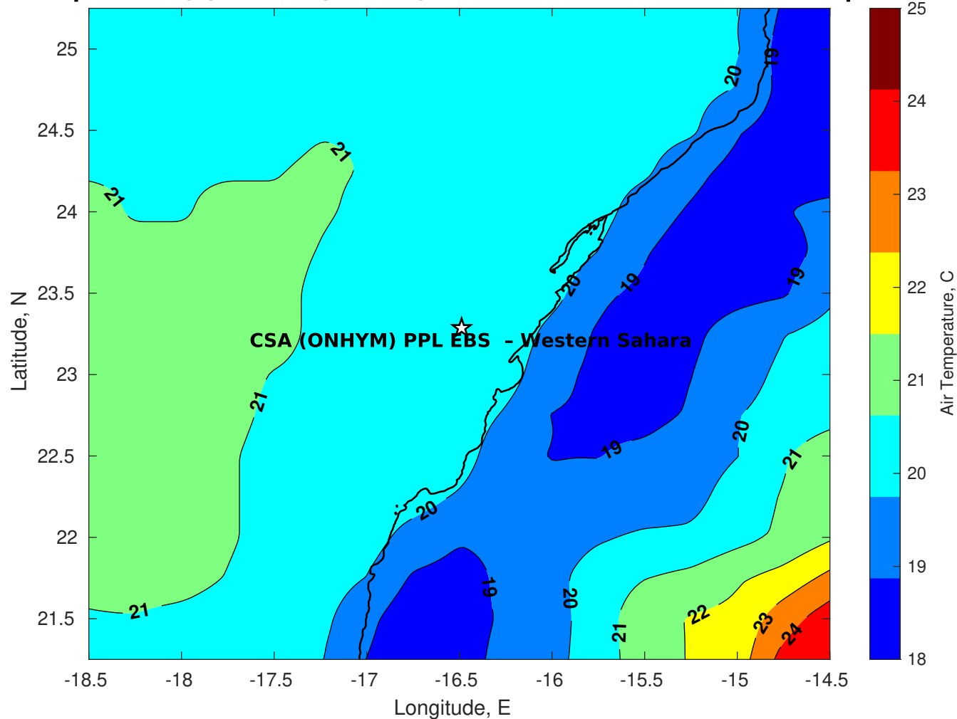
Air Temperature (C) for CSA (ONHYM) PPL EBS - Western Sahara at 13-Apr-2025
