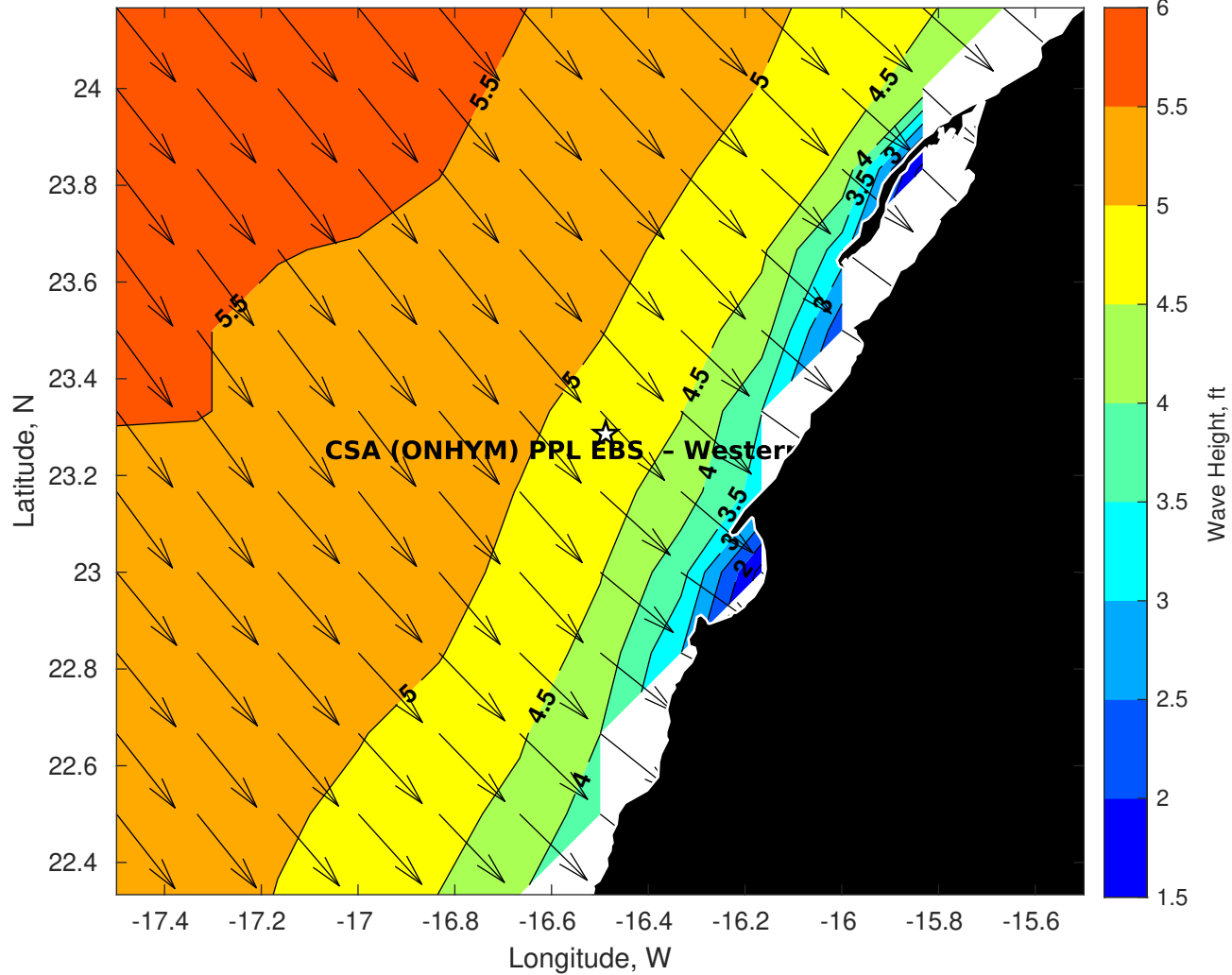
Wave Height (ft) for CSA (ONHYM) PPL EBS - Western Sahara at 13-Apr-2025 09:00:00
