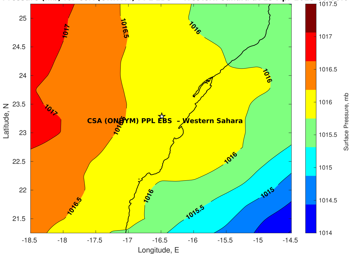
Surface Pressure (mb) for CSA (ONHYM) PPL EBS - Western Sahara at 13-Apr-2025 00:00:00
