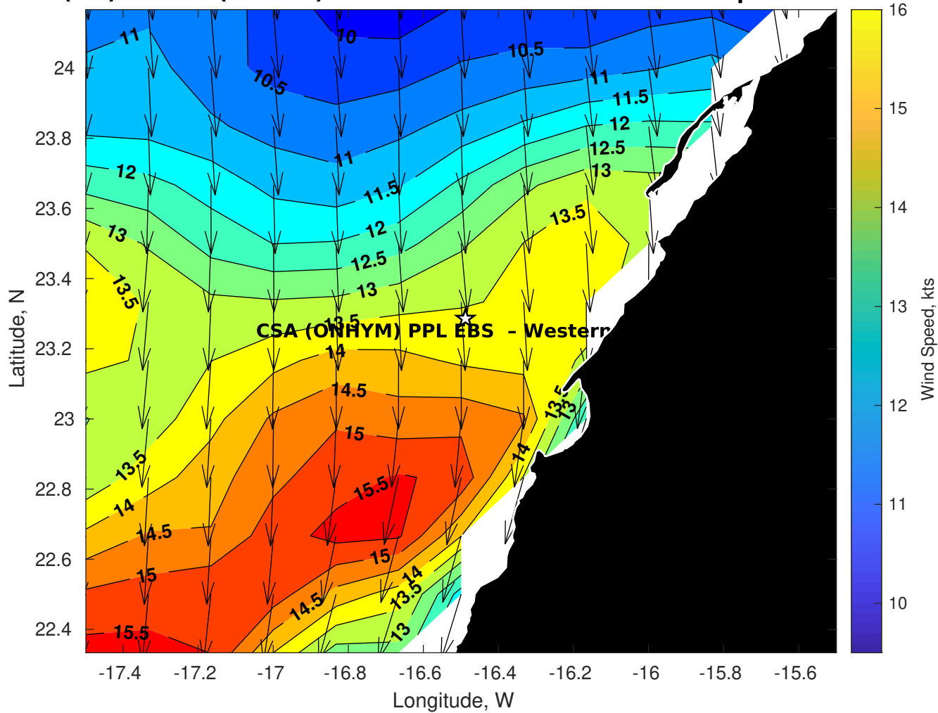
Winds (kts) for CSA (ONHYM) PPL EBS - Western Sahara at 13-Apr-2025 09:00:00
