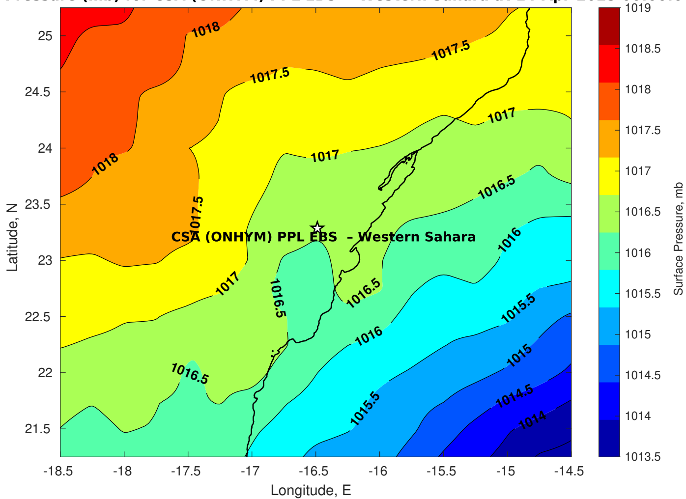
Surface Pressure (mb) for CSA (ONHYM) PPL EBS - Western Sahara at 14-Apr-2025 00:00:00
