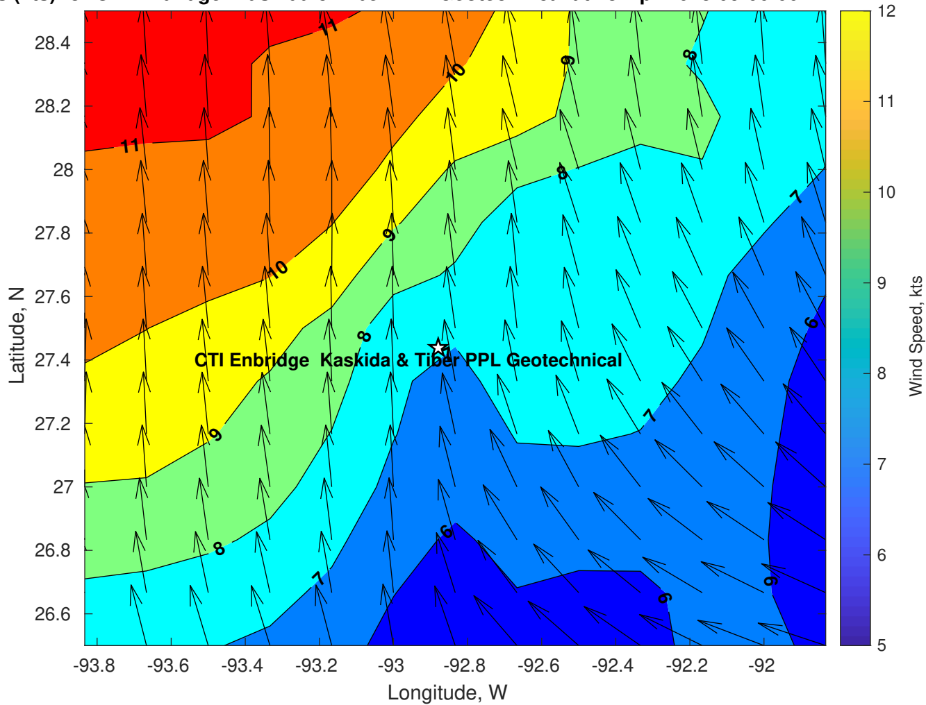
Winds (kts) for CTI Enbridge Kaskida & Tiber PPL Geotechnical at 13-Apr-2025 09:00:00
