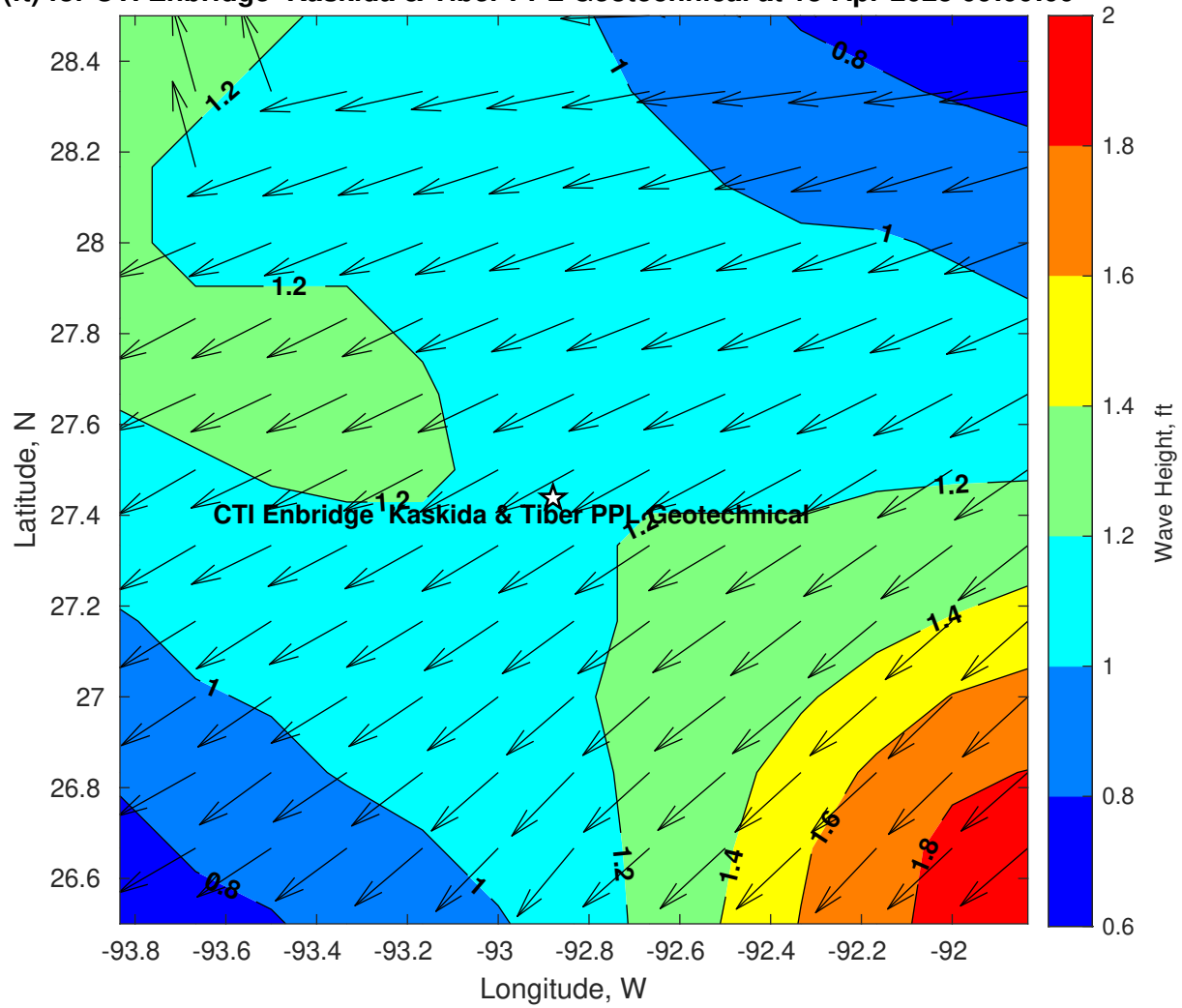
Wave Height (ft) for CTI Enbridge Kaskida & Tiber PPL Geotechnical at 13-Apr-2025 09:00:00
