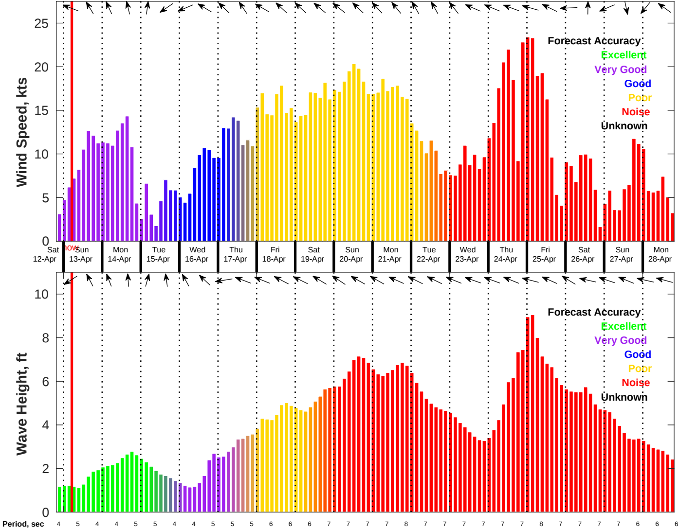
Wind & Wave Forecast for CTI Enbridge Kaskida & Tiber PPL Geotechnical from 12-Apr-2025 20:00:00 to 28-Apr-2025 20:00:00
