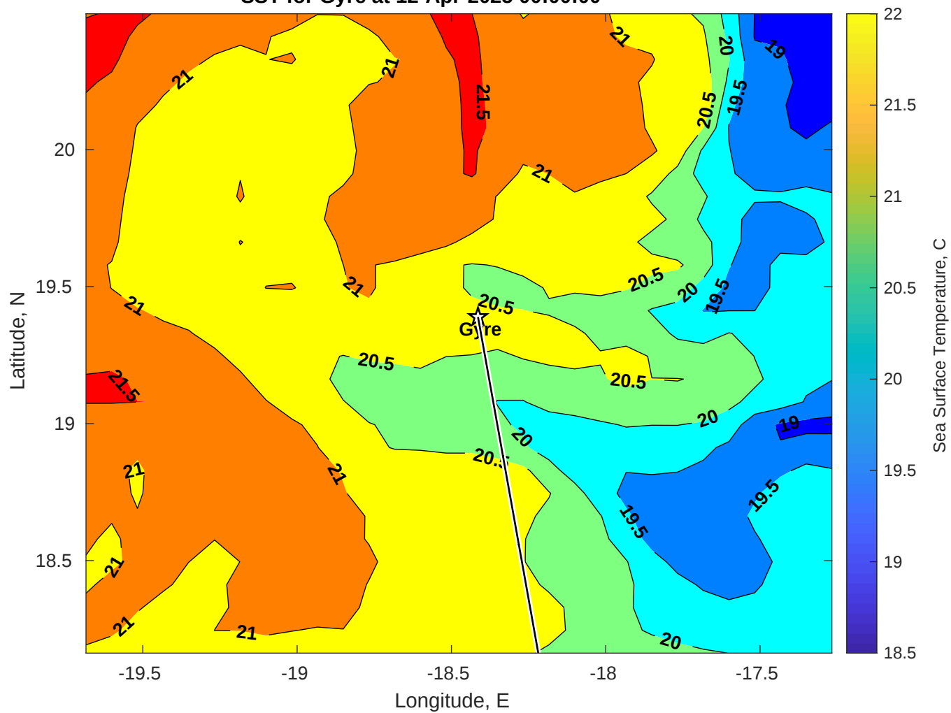
SST for Gyre at 12-Apr-2025 00:00:00
