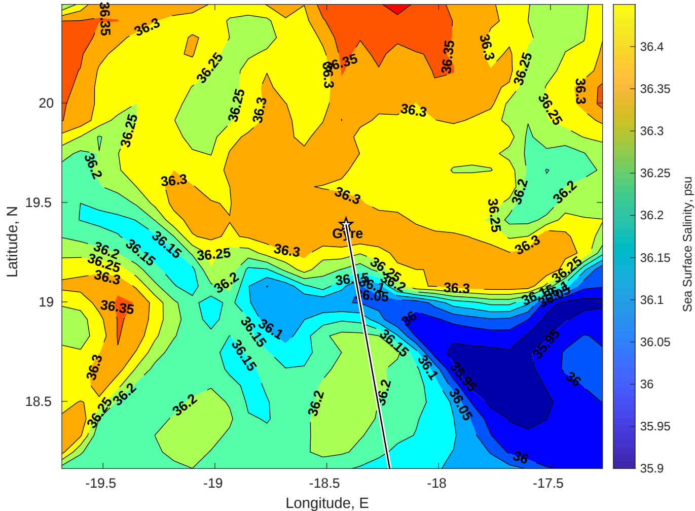
Surface Salinity for Gyre at 12-Apr-2025 00:00:00
