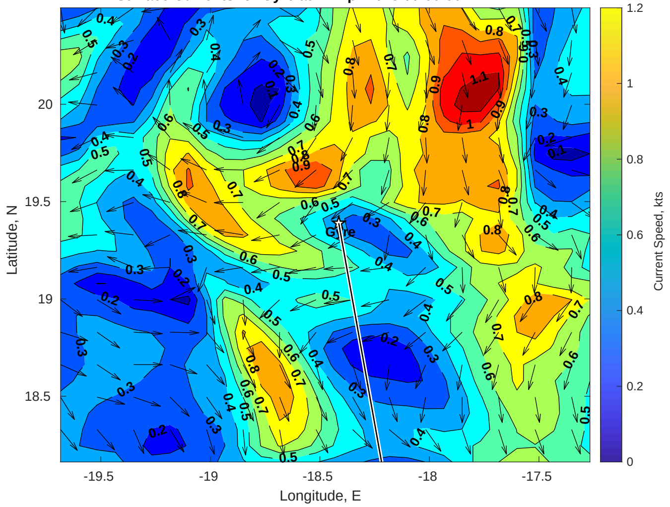
Surface Currents for Gyre at 12-Apr-2025 00:00:00
