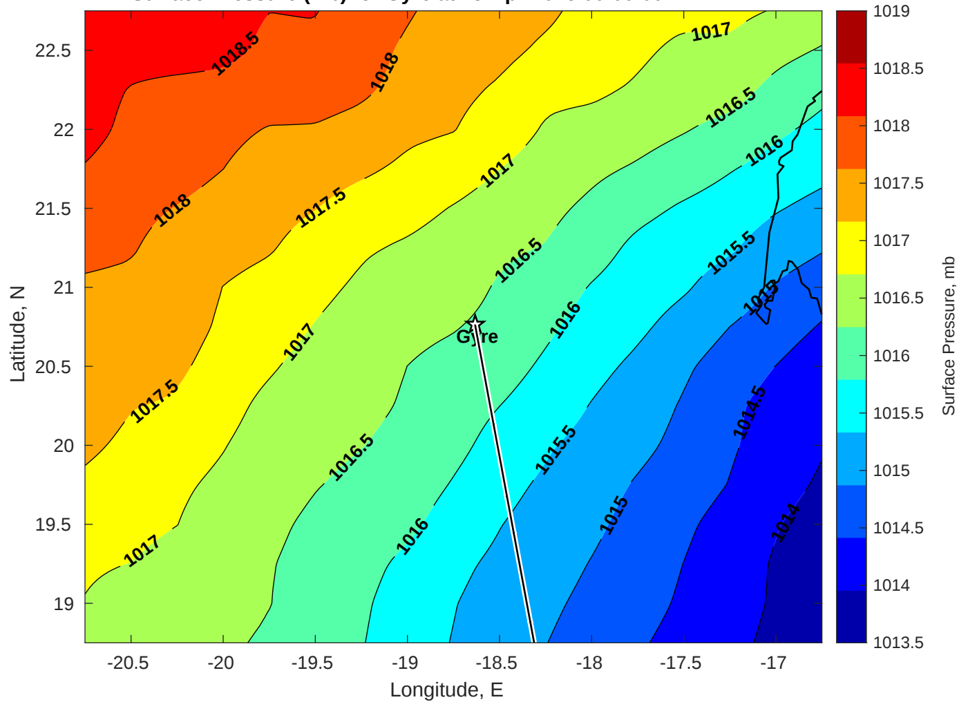
Surface Pressure (mb) for Gyre at 15-Apr-2025 00:00:00
