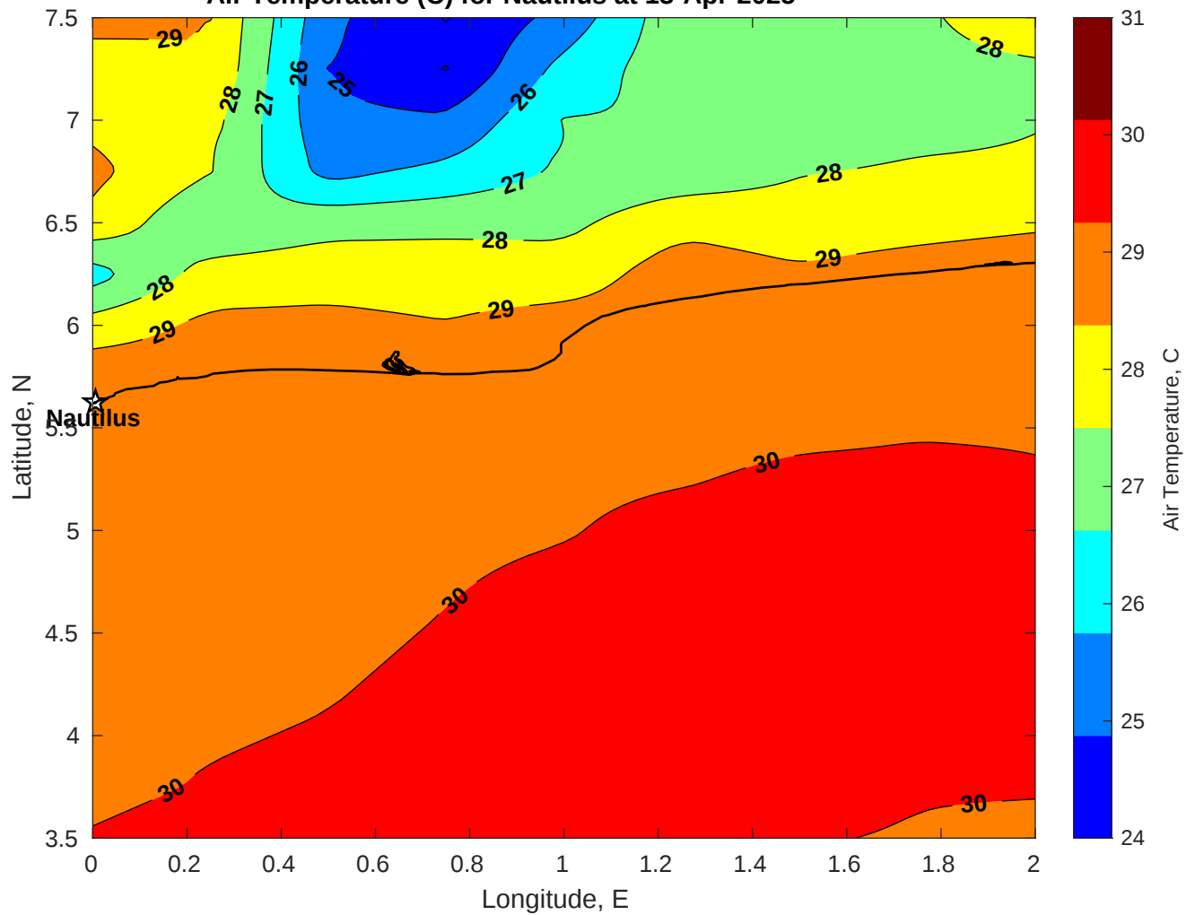
Air Temperature (C) for Nautilus at 13-Apr-2025
