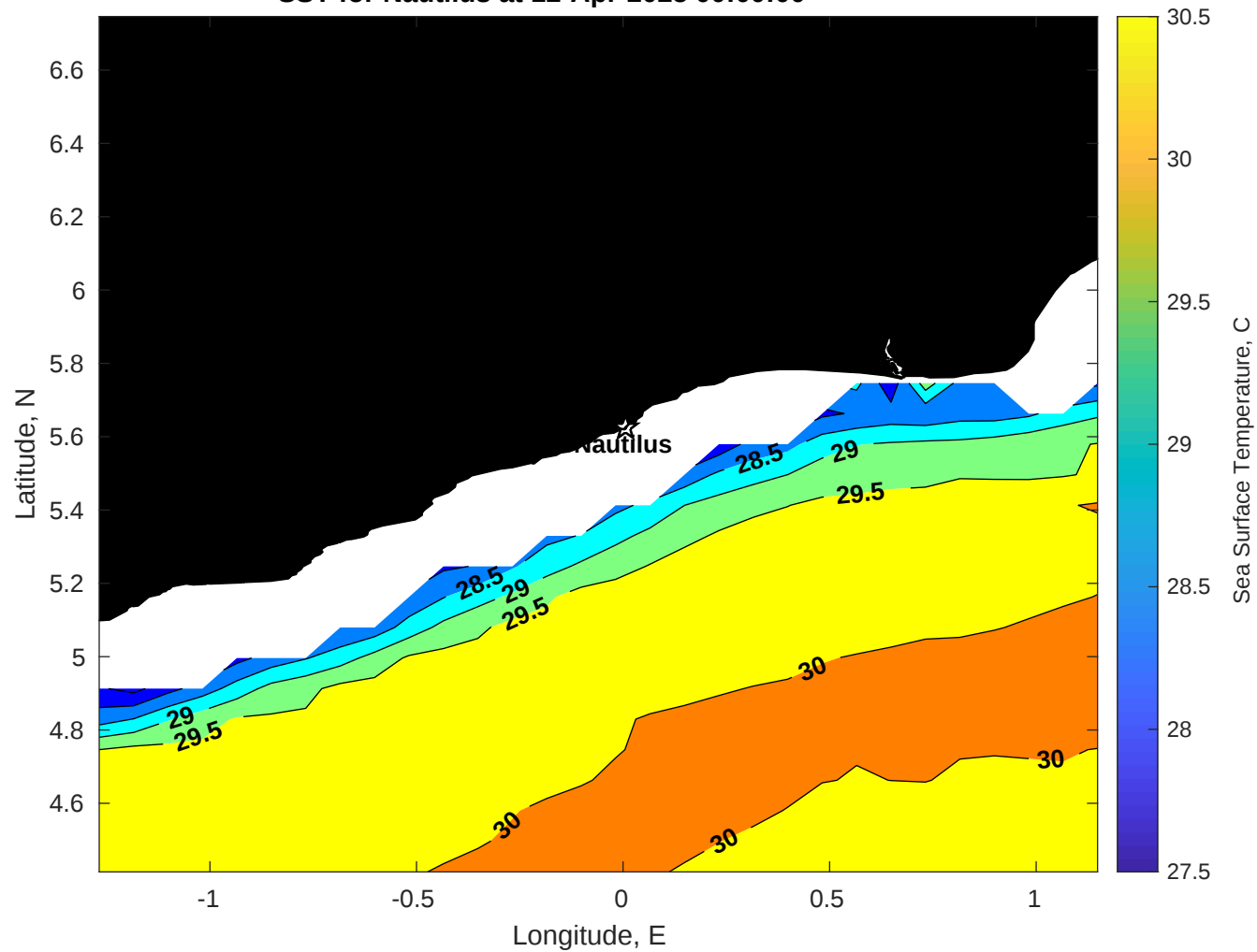
SST for Nautilus at 12-Apr-2025 00:00:00
