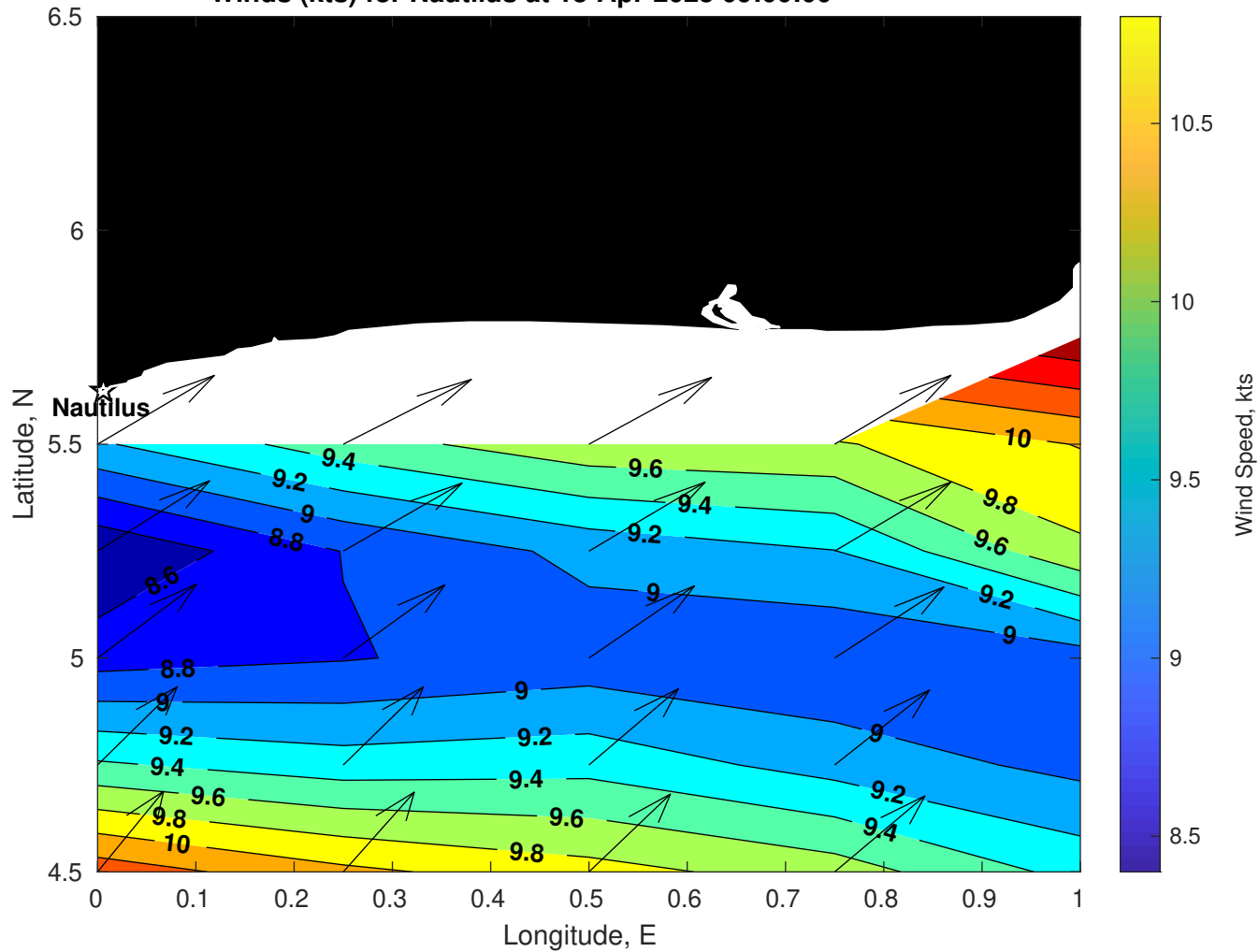
Winds (kts) for Nautilus at 13-Apr-2025 09:00:00
