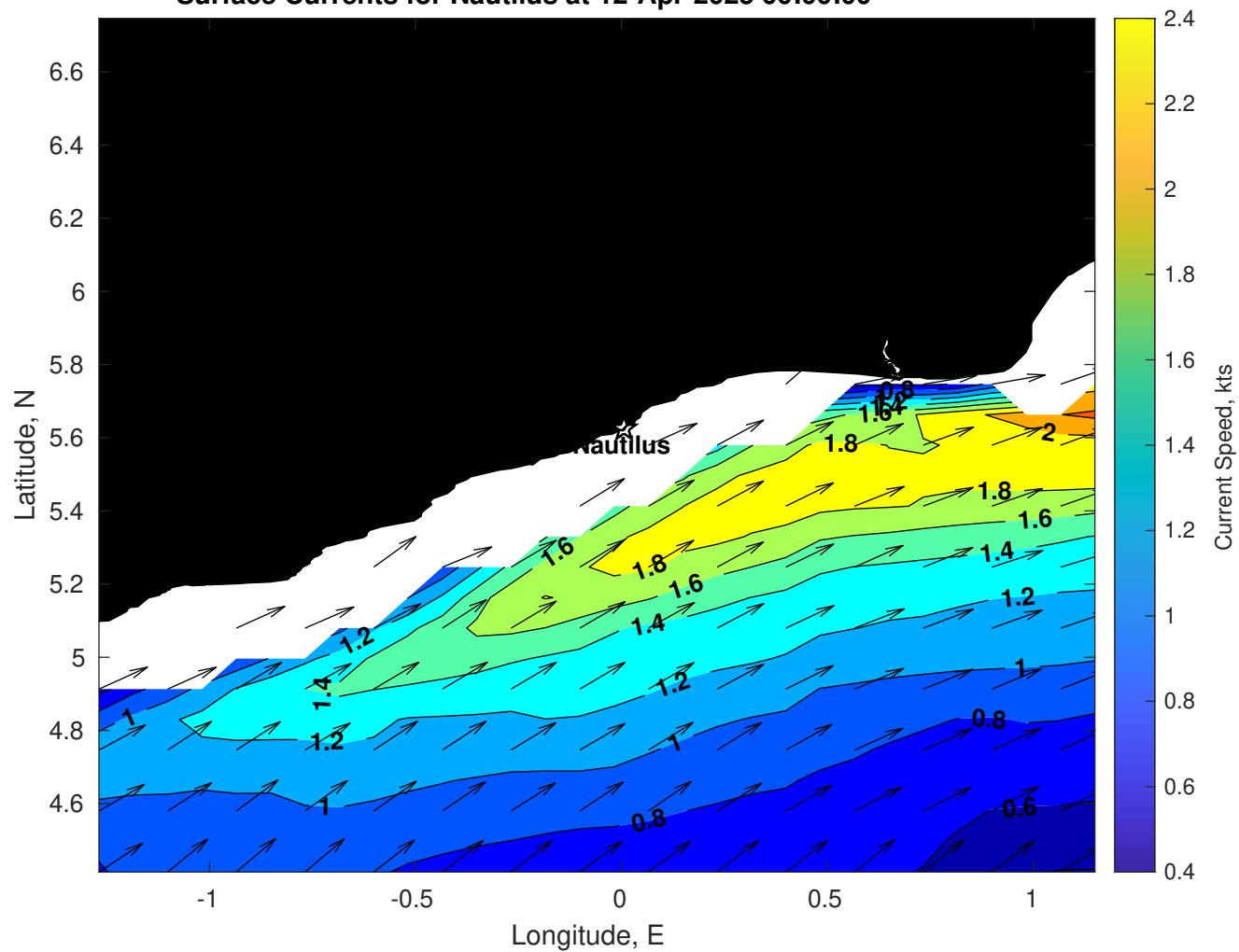
Surface Currents for Nautilus at 12-Apr-2025 00:00:00
