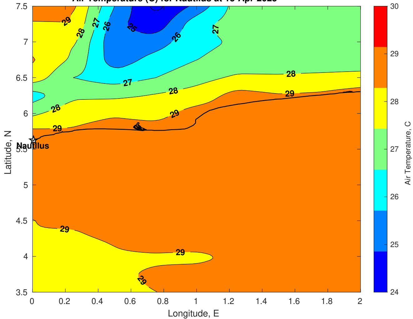
Air Temperature (C) for Nautilus at 13-Apr-2025
