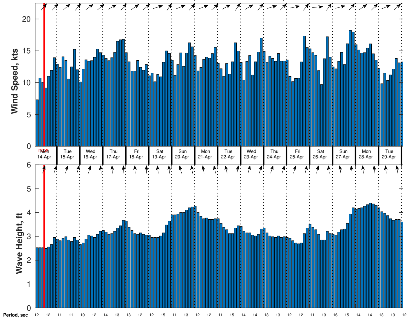
Wind & Wave Forecast for Nautilus from 13-Apr-2025 02:00:00 to 29-Apr-2025 02:00:00
