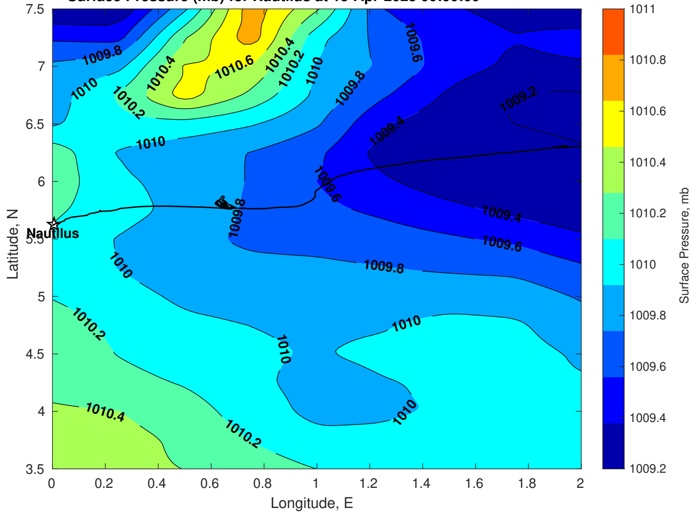
Surface Pressure (mb) for Nautilus at 15-Apr-2025 00:00:00
