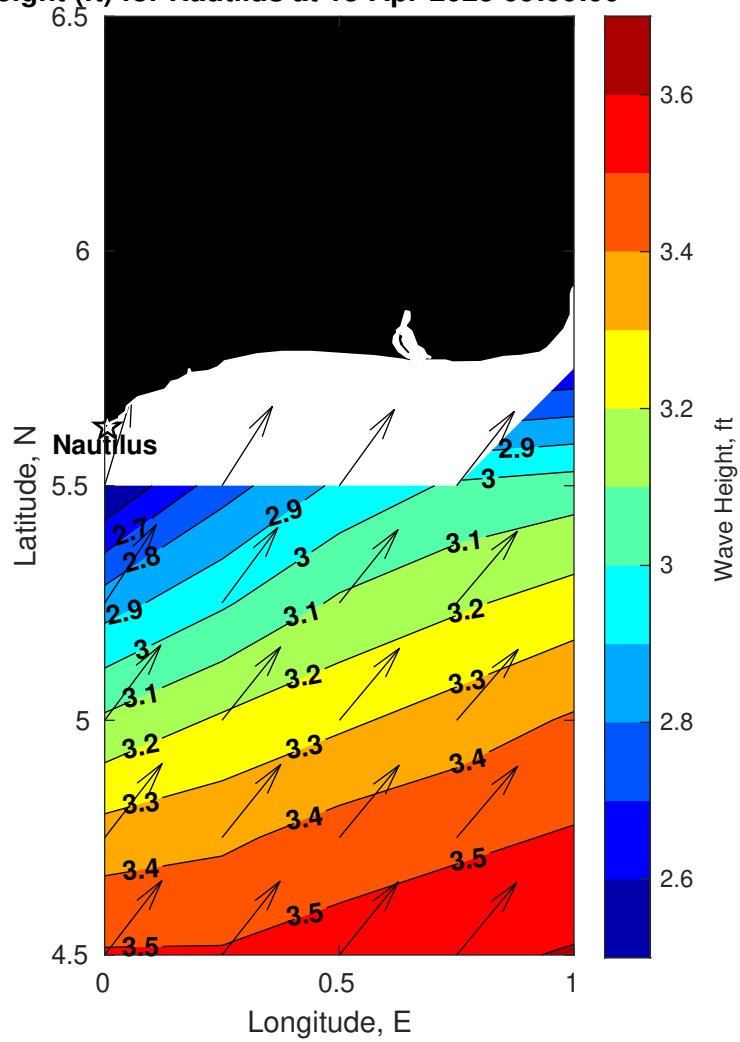
Wave Height (ft) for Nautilus at 13-Apr-2025 09:00:00
