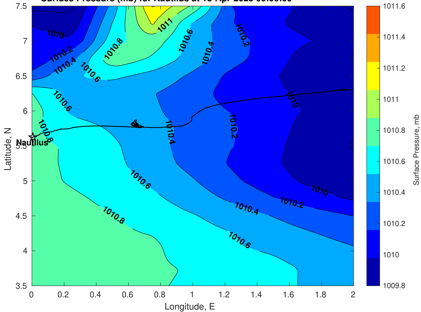
Surface Pressure (mb) for Nautilus at 13-Apr-2025 00:00:00
