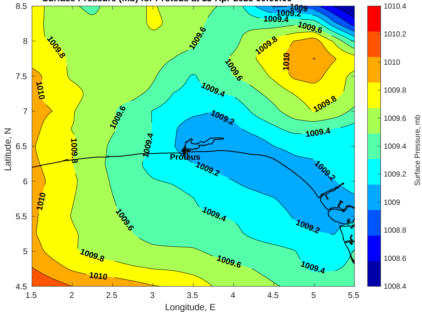
Surface Pressure (mb) for Proteus at 13-Apr-2025 00:00:00
