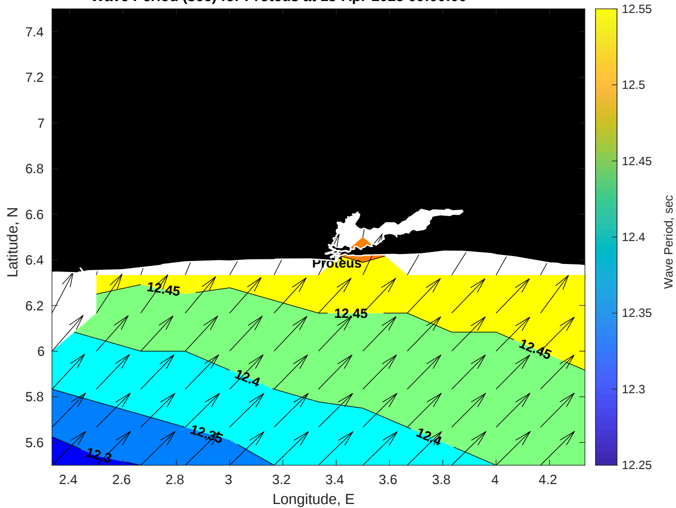
Wave Period (sec) for Proteus at 13-Apr-2025 09:00:00
