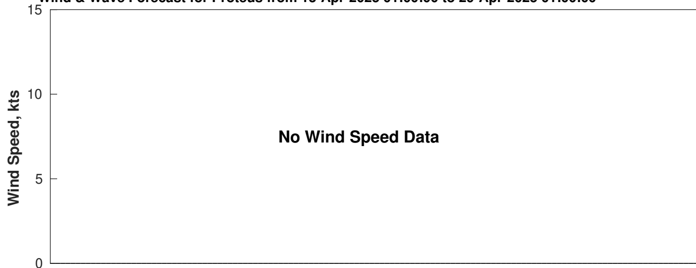
Wind & Wave Forecast for Proteus from 13-Apr-2025 01:00:00 to 29-Apr-2025 01:00:00
