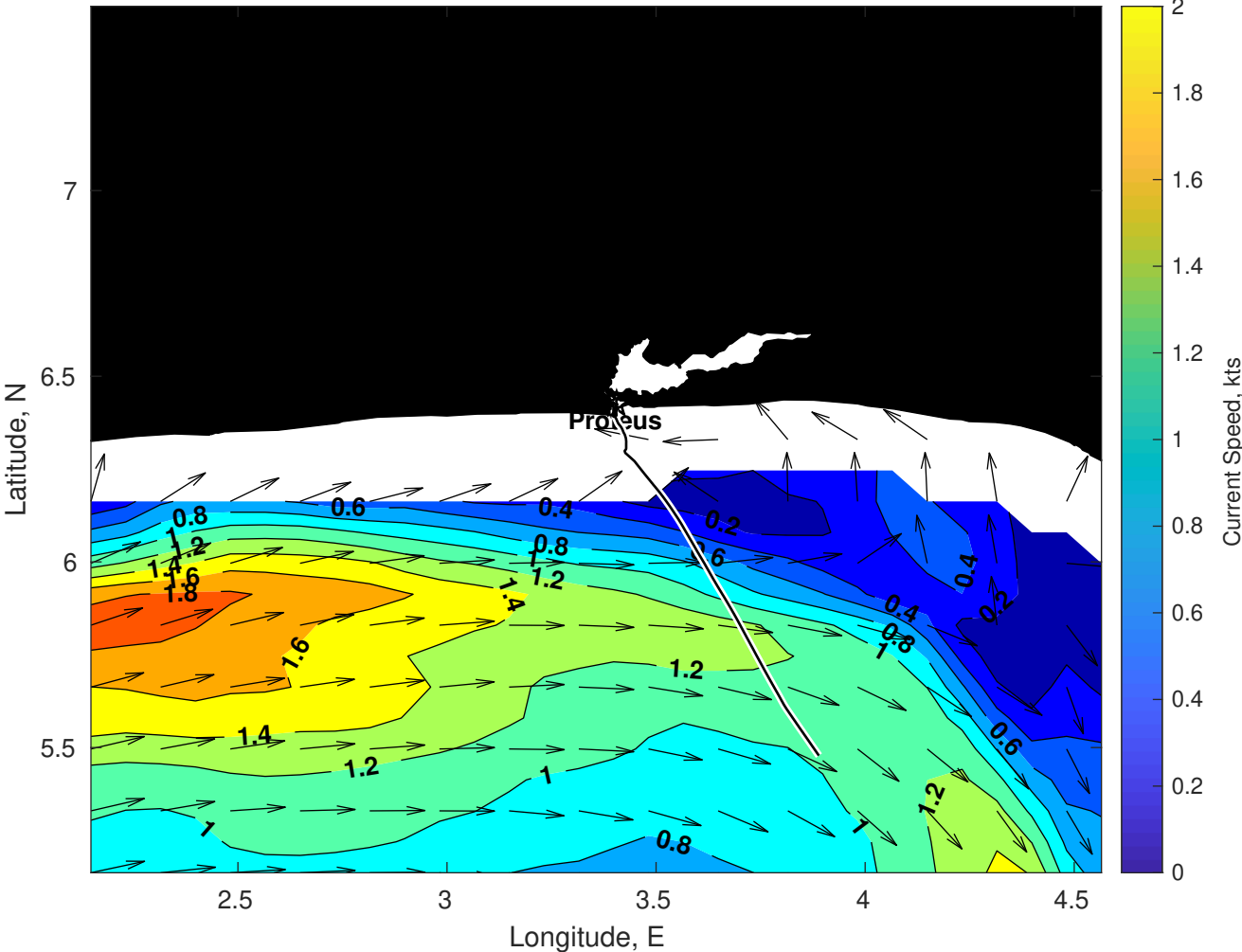
Surface Currents for Proteus at 12-Apr-2025 00:00:00
