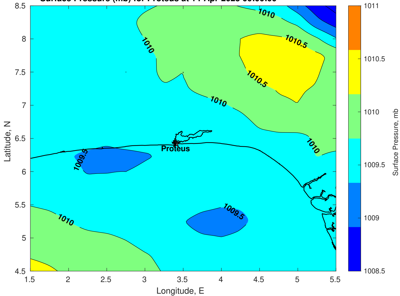
Surface Pressure (mb) for Proteus at 14-Apr-2025 00:00:00
