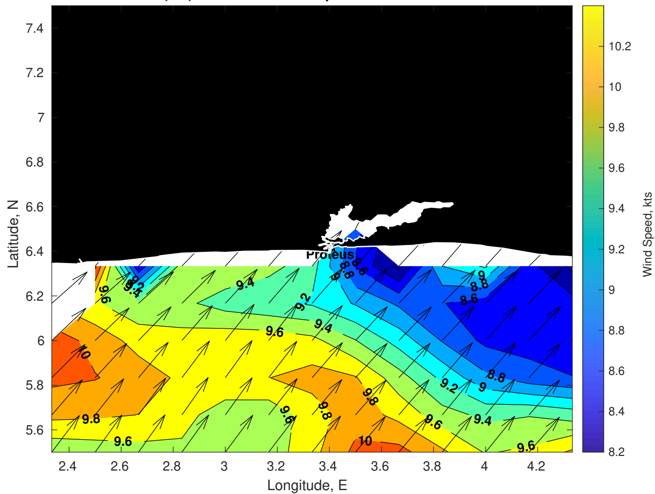
Winds (kts) for Proteus at 13-Apr-2025 09:00:00
