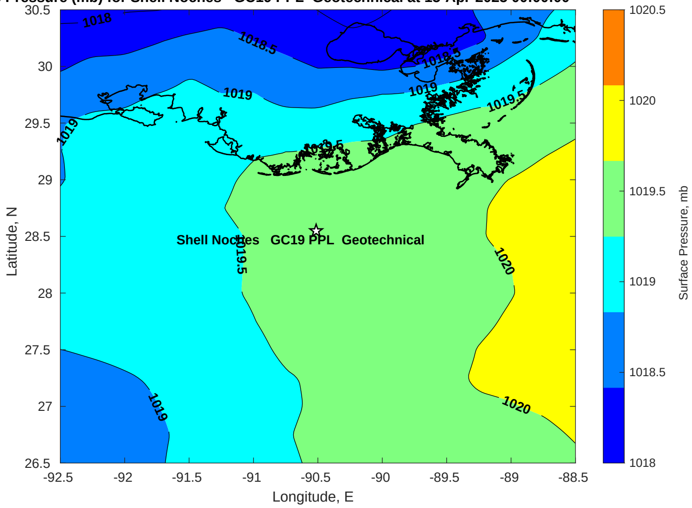
Surface Pressure (mb) for Shell Noches GC19 PPL Geotechnical at 15-Apr-2025 00:00:00
