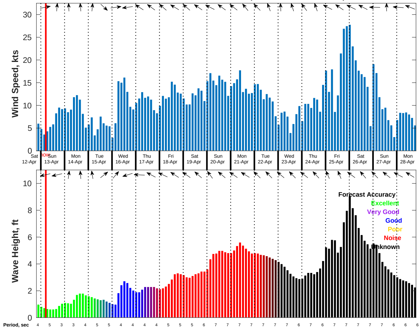
Wind & Wave Forecast for Shell Noches GC19 PPL Geotechnical from 12-Apr-2025 20:00:00 to 28-Apr-2025 20:00:00
