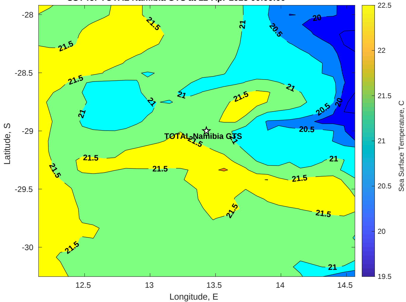
SST for TOTAL Namibia GTS at 12-Apr-2025 00:00:00
