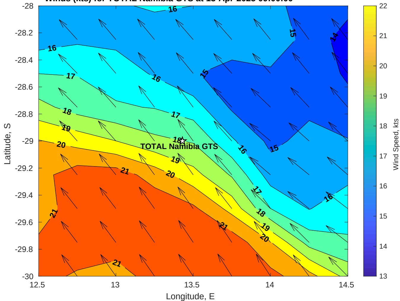
Winds (kts) for TOTAL Namibia GTS at 13-Apr-2025 09:00:00
