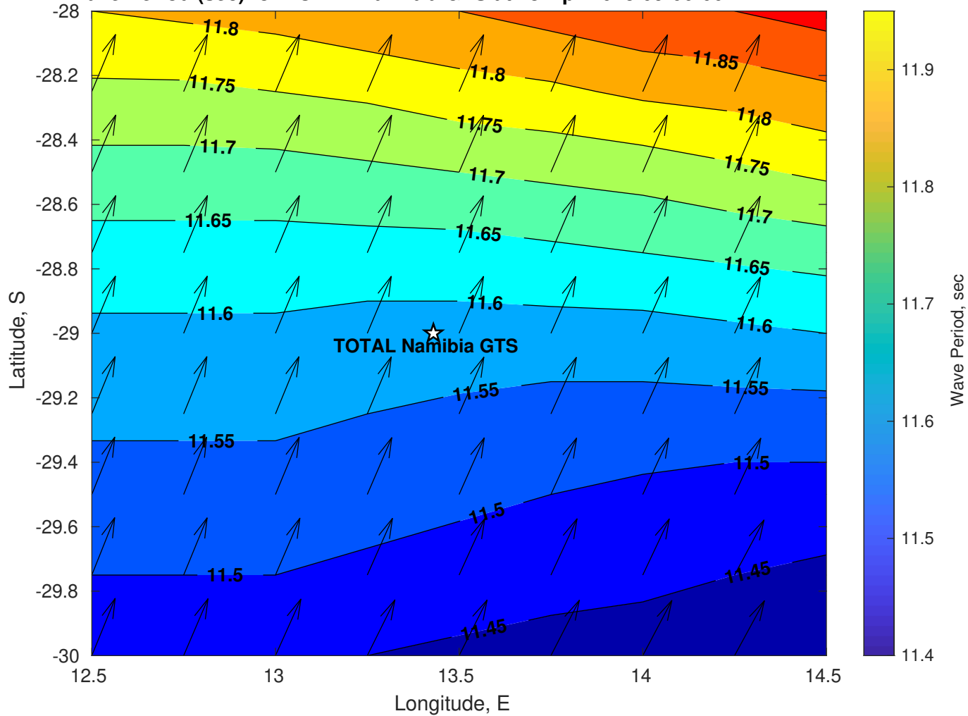
Wave Period (sec) for TOTAL Namibia GTS at 13-Apr-2025 09:00:00
