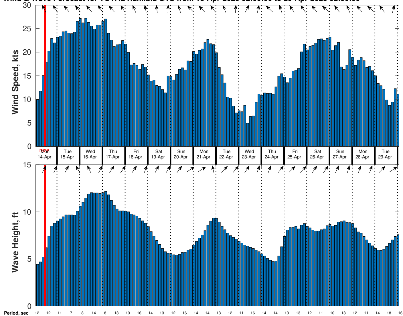
Wind & Wave Forecast for TOTAL Namibia GTS from 13-Apr-2025 02:00:00 to 29-Apr-2025 02:00:00
