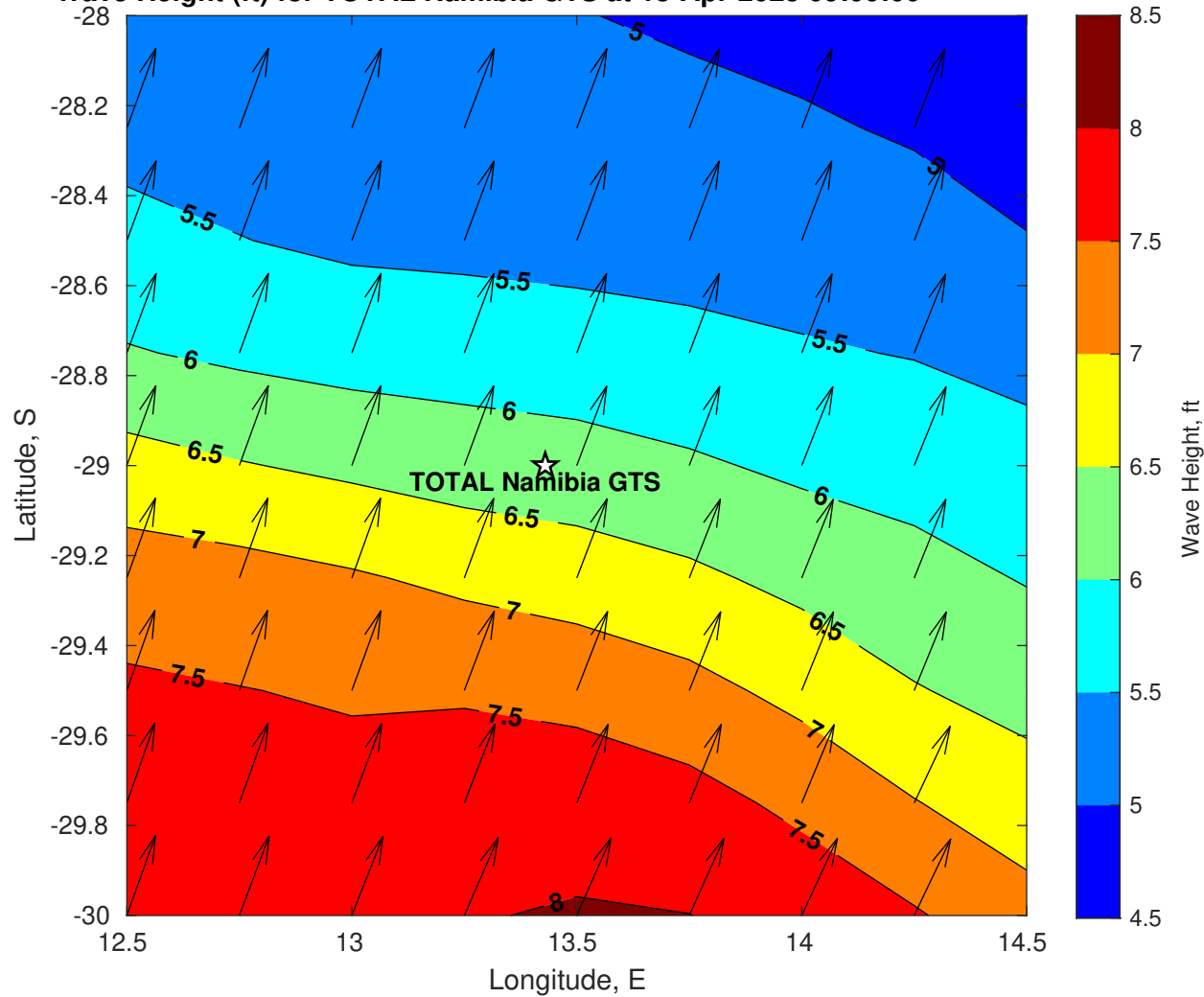
Wave Height (ft) for TOTAL Namibia GTS at 13-Apr-2025 09:00:00
