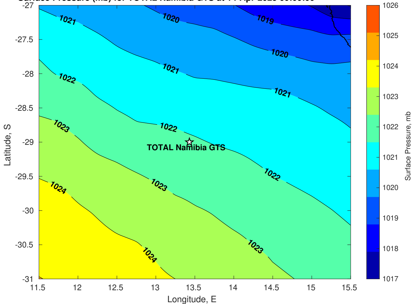
Surface Pressure (mb) for TOTAL Namibia GTS at 14-Apr-2025 00:00:00
