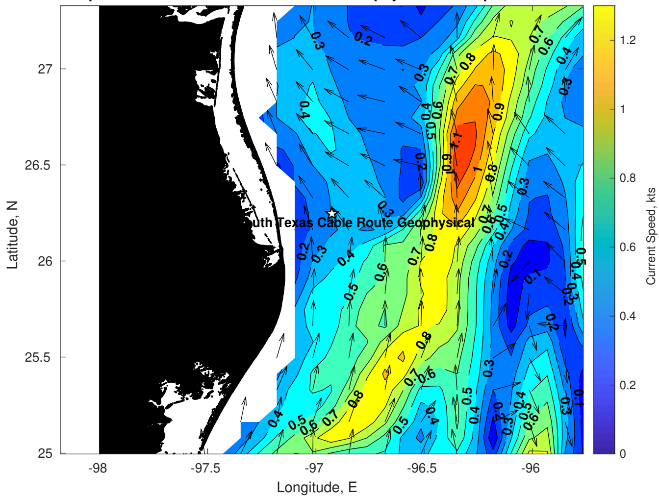
Surface Currents for Tampnet P2378 South Texas Cable Route Geophysical at 12-Apr-2025 00:00:00
