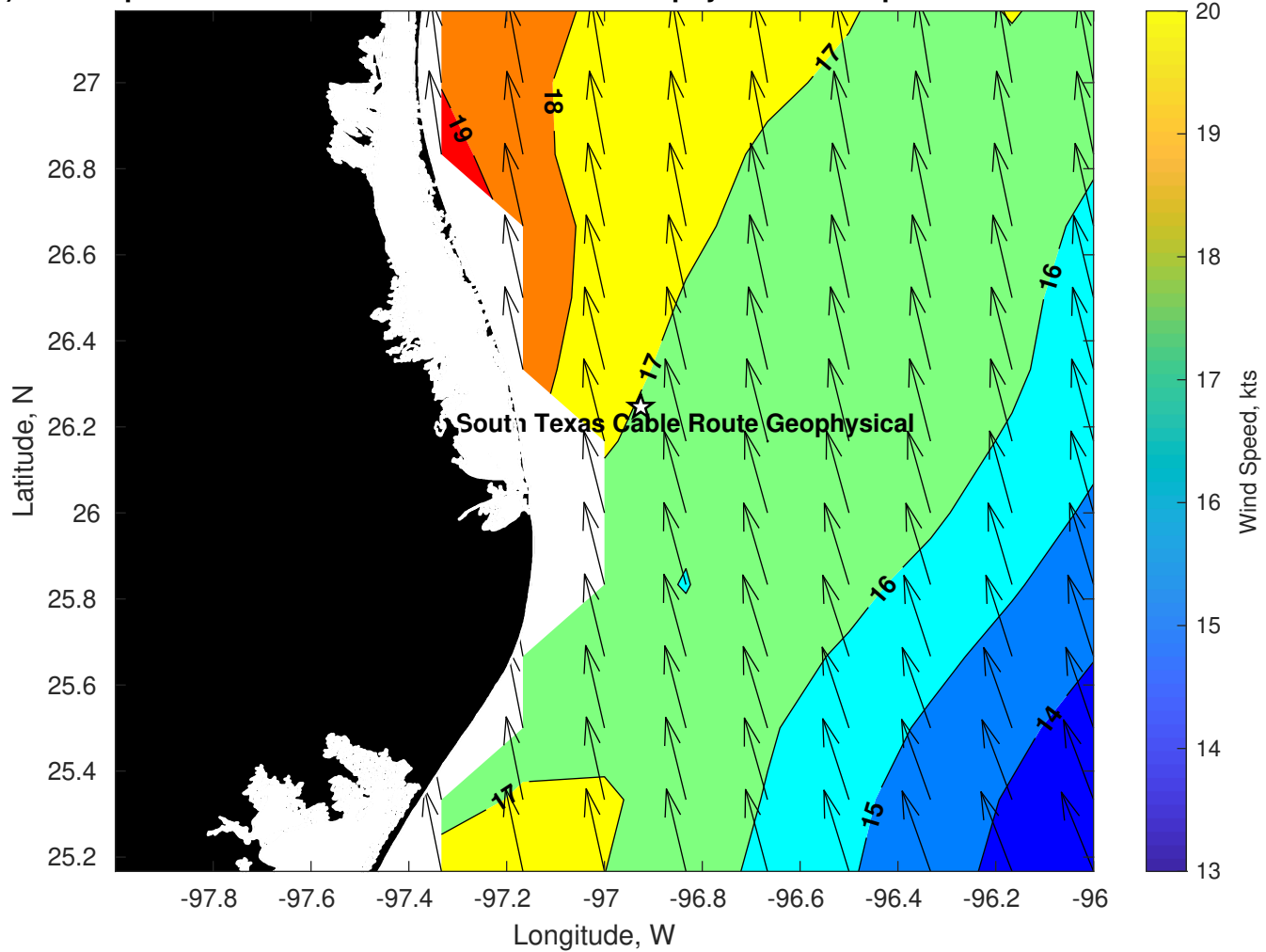
Winds (kts) for Tampnet P2378 South Texas Cable Route Geophysical at 13-Apr-2025 09:00:00
